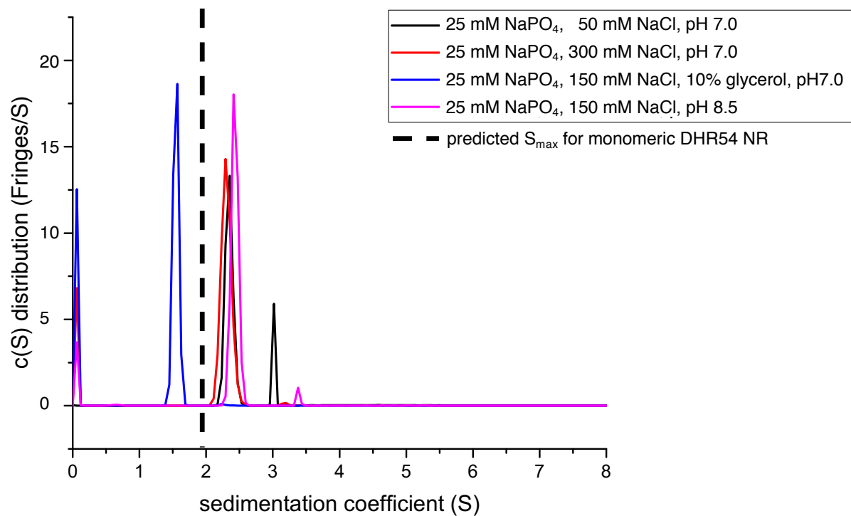
Supplemental Figure 1. Sedimentation Velocity c(S) plot for DHR54 NR in the absence and presence of glycerol. Data were processed and fitted in Sedfit 33 as previously described 4 . The predicted S_{max} (dotted vertical line) was calculated for DHR54 NR using Sednterp 34 . In the presence of 10 % glycerol, the c(S) distributions are consistent with monomers.
