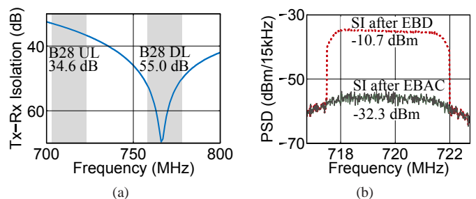
Fig. 6. (a) Measured passive Tx-Rx isolation provided by the EBD. (b) Measured Tx band SI (i.e. the Tx blocker) before and after AC.
