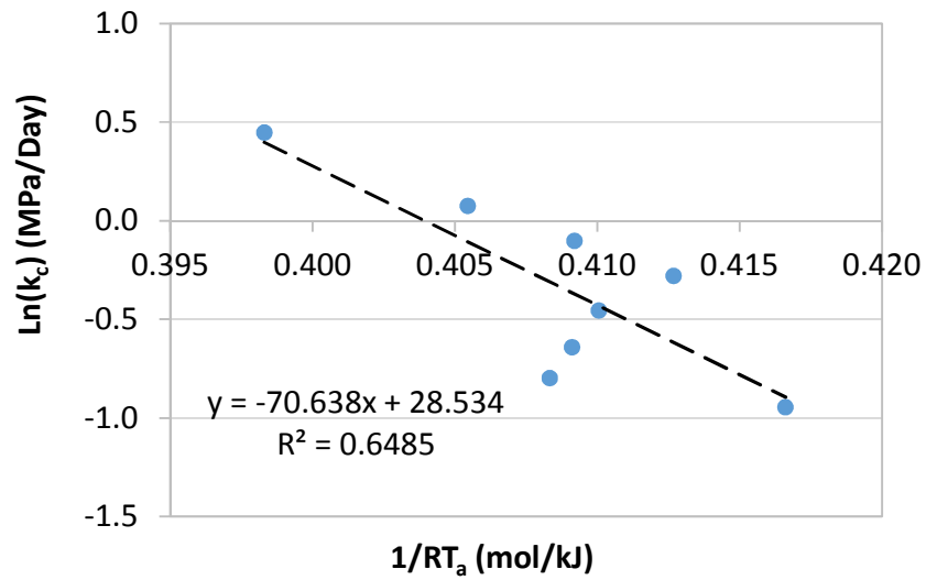
(b) E_2 of the overlay
