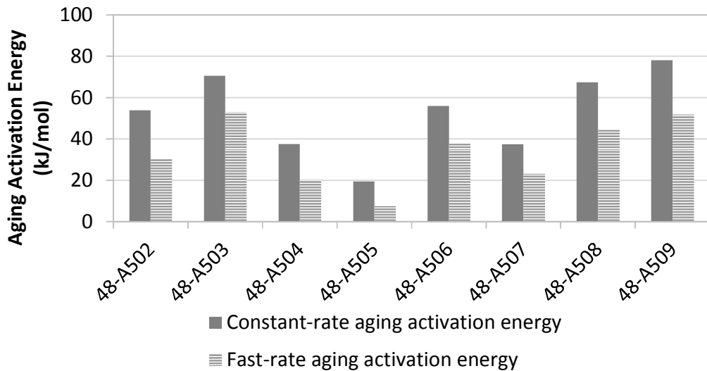
Figure 9. Calculated aging activation energies for all Texas SPS-5 sections
