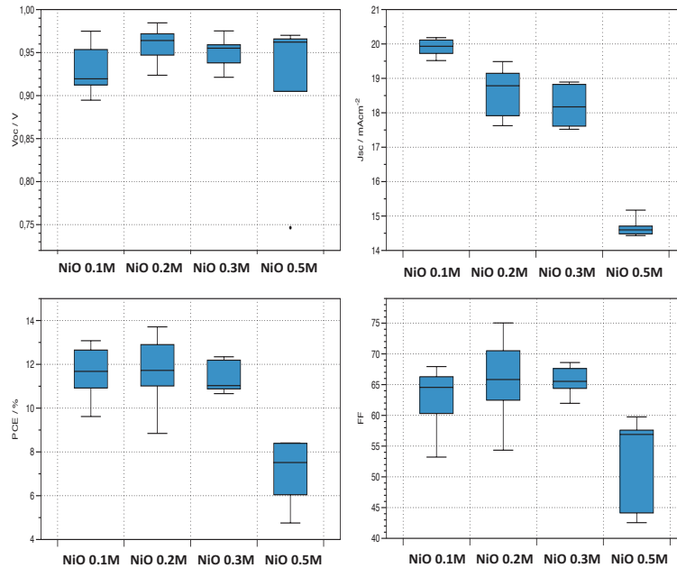
FIGURE 6. Statistics of the four main photovoltaic parameters for the PSCs differing in the type of NiO x -HTL.
