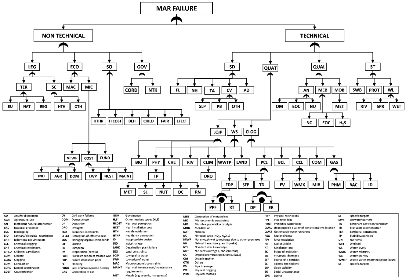
Figure 2. General fault tree for the operational phase.
