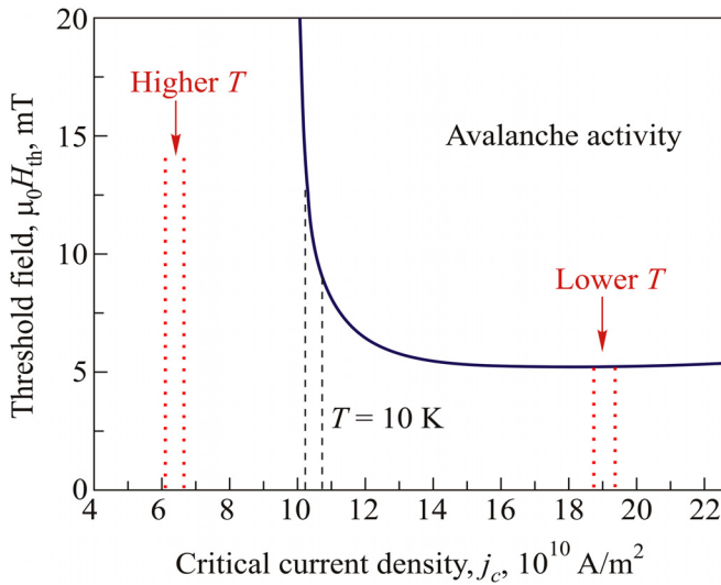
Fig. 15. Graph of the threshold perpendicular magnetic field versus critical current density, for onset of avalanche activity in films of \text{MgB}_2 (full curve). The pairs of dashed/dotted lines show the critical current density at 3 temperatures, and the two lines in each pair indicate the anisotropy in j_c .
