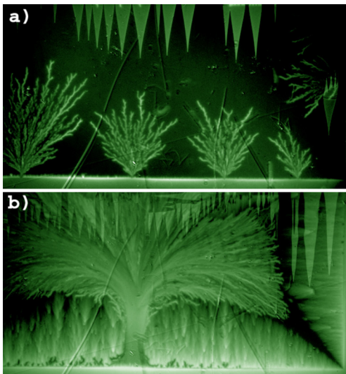
Fig. 4. Magneto-optical images of dendritic flux avalanches in a NbN film taken at (a) T = 4 K and (b) T = 6 K. The zigzag patterns are domain boundaries in the FGF. From Ref. 29.
