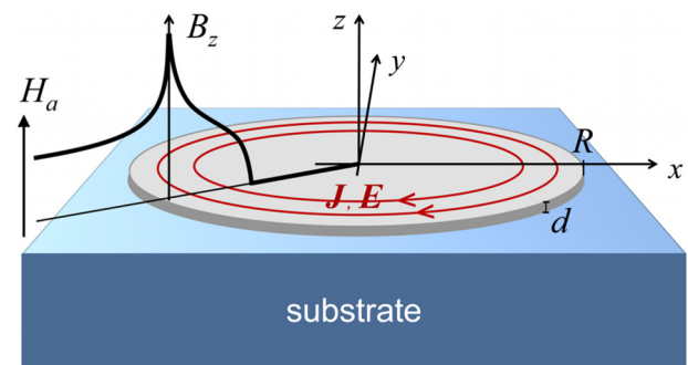
Fig. 9. Sample configuration. A thin superconducting disk on a substrate exposed to a gradually increasing perpendicular magnetic field, H_a . The flux density, B_z , is advancing from the edge along with a distribution of induced shielding current, J , and electrical field, E . From Ref. 63.
