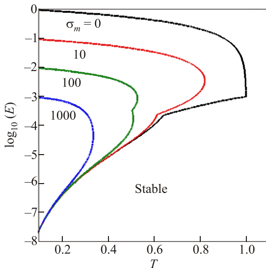
Fig. 7. The lines show the boundary of the instability region when changing the normal metal conductivity \sigma_m = 0, 10, 100, and 1000 . Increasing metal layer conductivity improves stability at high E and T . Parameters are \alpha = 10^{-5}, \beta = 0.1, \gamma = 10, t_x = 0.1, n_1 = 20 .
