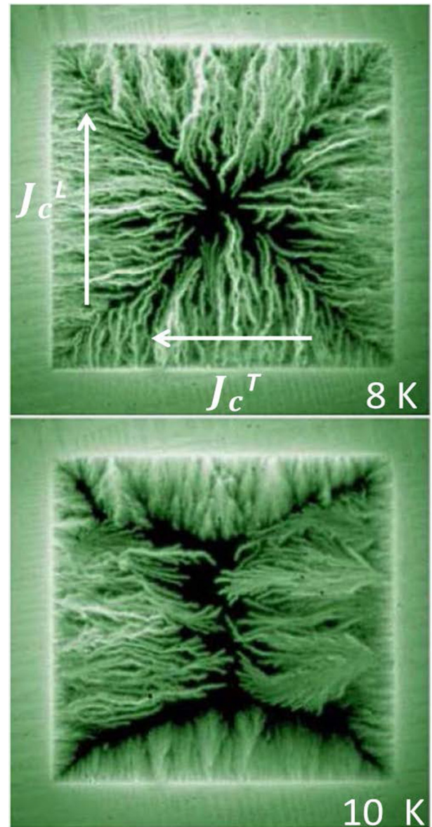
Fig. 14. Magneto-optical images of flux penetration in a 200 nm thick MgB 2 film grown on a vicinal substrate. The steps in the substrate are aligned approximately vertical in the figure. The upper and lower images were recorded at 8 and 10 K, respectively. The non-uniformity in the penetration at 10 K from the two horizontal edges is due to edge roughness and other minor sample imperfections. Adapted from Ref. 69.
