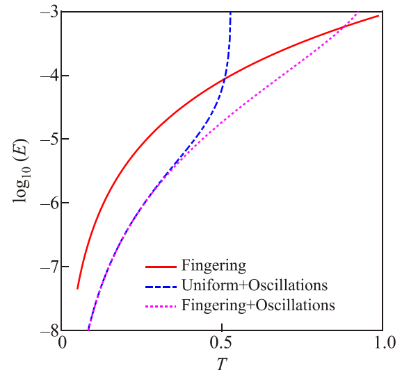
Fig. 6. The threshold for onset of instability in the T - E plane, for the fingering, fingering + oscillatory, and uniform + oscillatory conditions. In a uniform sample, the lowest of these curves determines the onset of instability. The parameters are \alpha = 10^{-5} , \beta = 0.1 , \gamma_0 = 10 , l_x = 0.1 , n_1 = 50 .
