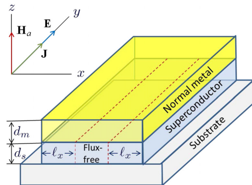
Fig. 5. Sketch of the system: a thin superconducting strip of thickness d_s with a deposited metal layer of thickness d_m . The superconductor is in thermal contact with the substrate, kept at constant temperature T_0 , but not with the metal. Current flows in the y direction and flux has penetrated a distance l_x from both sides due to the applied magnetic field H_a .
