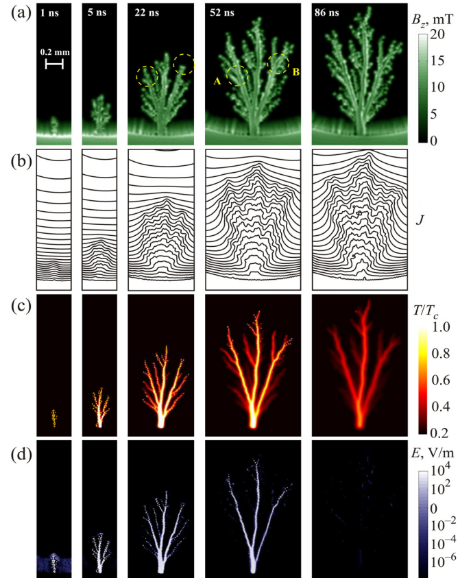
Fig. 11. Evolution of a breakdown event. (a) Distributions of the magnetic flux density B_z , (b) the induced sheet current J , (c) the temperature T , and (d) the electrical field E , at times t = 1, 5, 22, 52 and 86 ns after nucleation of the thermo-electromagnetic instability.
