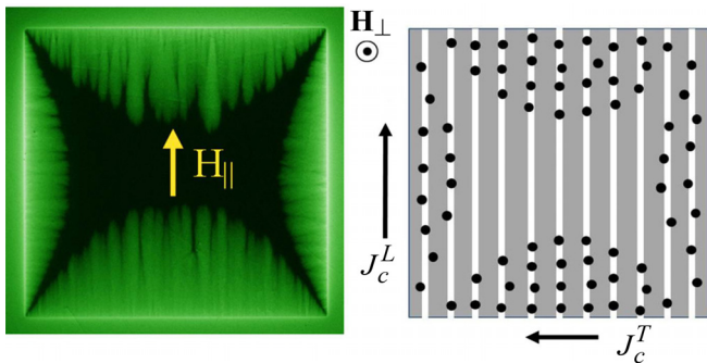
Fig. 16. Left: Magneto-optical image showing field-induced anisotropic flux penetration in a 2.5 \times 2.5 mm Nb film of thickness 200 nm. The in-plane field H_{\parallel} = 1 kOe was frozen in during the initial cooling to 7 K. From Ref. 88. Right: Illustration of anisotropic penetration of perpendicular vortices (black dots) in the presence of frozen-in in-plane vortices (white lines). From Ref. 88.
