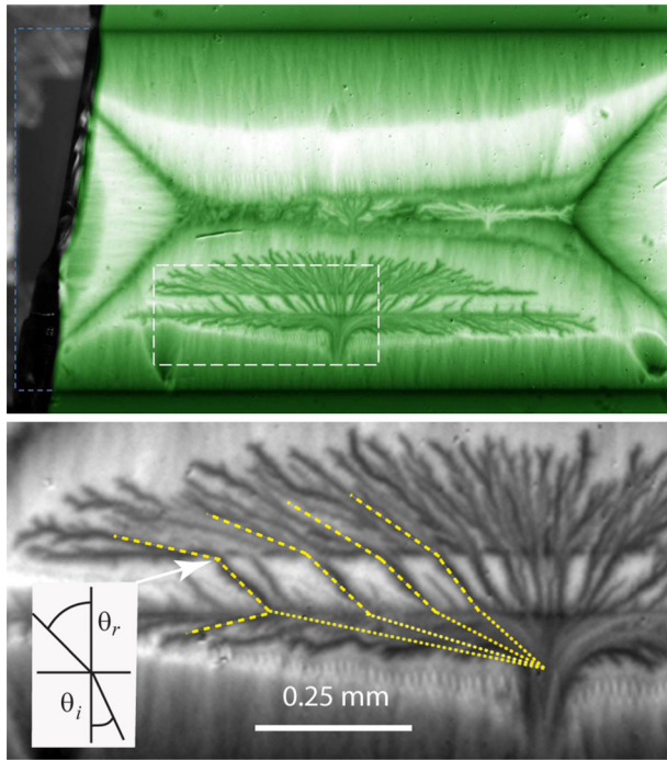
Fig. 13. Magneto-optical image of a flux avalanche occurring at 3.7 K in the metal coated NbN film. The image covers the lower central part of the film, and was recorded in the remnant state after the field was first raised to 17 mT. The horizontal bright strip permeated by dark line segments is the metal coated strip located nearest to the sample center. The strip near the edge is invisible, as the avalanche crossed this region through a single channel perpendicular to the edge. From Ref. 39.
