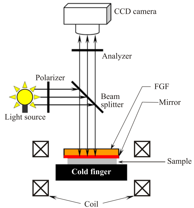
Fig. 3. Schematic of a typical MOI setup. A sample is mounted on a cold finger of a liquid He flow cryostat. Resistive coils are used as a source of an external magnetic field. The light from a mercury lamp shines through a polarizer and is guided onto an indicator film, where it experiences Faraday rotation. The light is reflected by a mirror and passes an analyzer before hitting a CCD matrix of a computer-operated camera. From Ref. 29.
