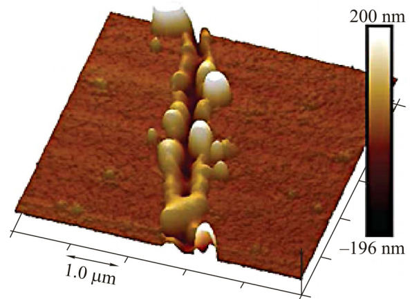
Fig. 2. Height profile plot obtained by AFM scan of a \text{YBa}_2\text{Cu}_3\text{O}_x film after being exposed to a rapidly increasing perpendicular applied magnetic field. From Ref. 24.
