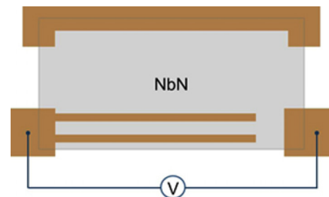
Fig. 12. Schematics of the rectangular NbN superconducting film covered by a Cu-layer patterned as seen in the figure. Shown is also the voltage pulse measurement circuit, which allows time-resolved observation of the avalanches starting from the lower film edge. From Ref. 39.
