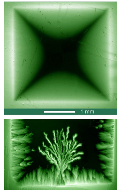
Fig. 1. Upper panel: Magneto-optical image of the magnetic flux distribution in a square film of \text{YBa}_2\text{Cu}_3\text{O}_x exposed to a perpendicular magnetic field of 20 mT. Lower panel: Flux distribution in a \text{MgB}_2 film after a dendritic avalanche occurred from the lower edge. The image brightness represents perpendicular component of the magnetic induction, B_z .
