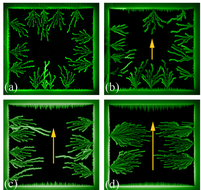
Fig. 18. Magneto-optical images of the penetration of perpendicular flux in a square Nb film, where in-plane fields, indicated by the arrows, were applied during the initial cooling to 2.5 K. In panels (a)–(d) the H_{\parallel} were 0, 0.7, 1.0 and 1.5 kOe, respectively. From Ref. 88.
