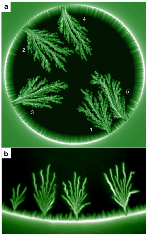
Fig. 10. Flux density after a few breakdown events. (a) Simulated distribution of B_z in a superconducting disk after five flux avalanches occurred in the sequence indicated by the numbers as the applied field was ramped up from zero to \mu_0 H_a = 8.5 mT. (b) Magneto-optical image of the flux density in a superconducting \text{MgB}_2 film cooled to 6 K and then exposed to an applied field of 3.8 mT. From Ref. 63.
