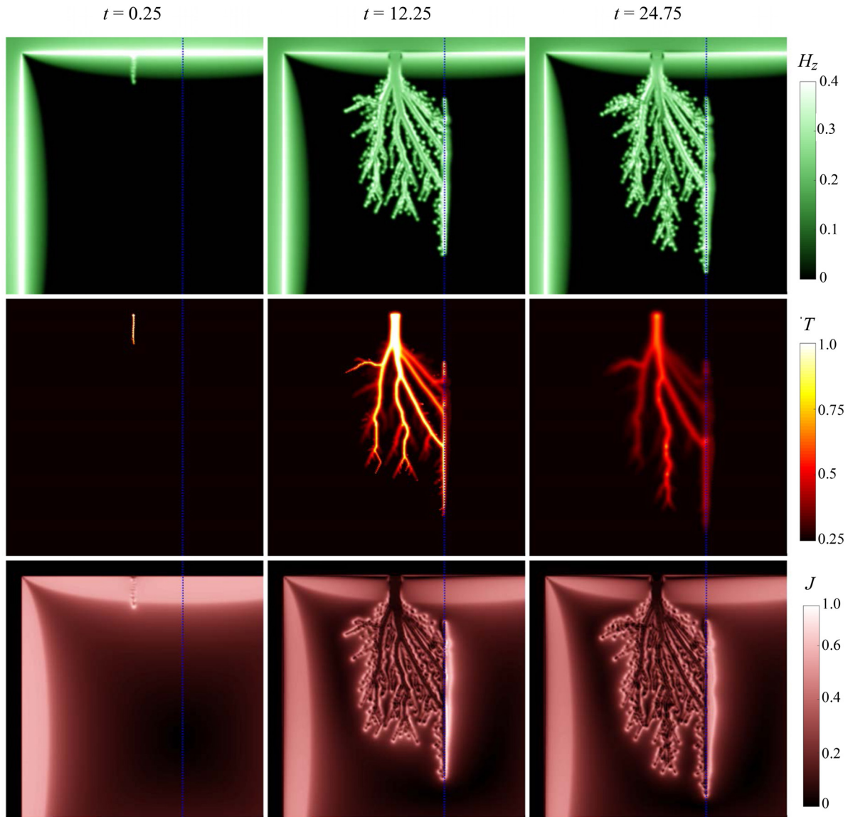
Fig. 8. Simulated evolution of an avalanche in a sample where the region to the right of the dotted line is covered with metal with \sigma_m = 1000 . Distributions of the magnetic field H_z , temperature T and sheet current magnitude J , at times t = 0.25 , 12.25 and 24.75 after nucleation of the avalanche.
