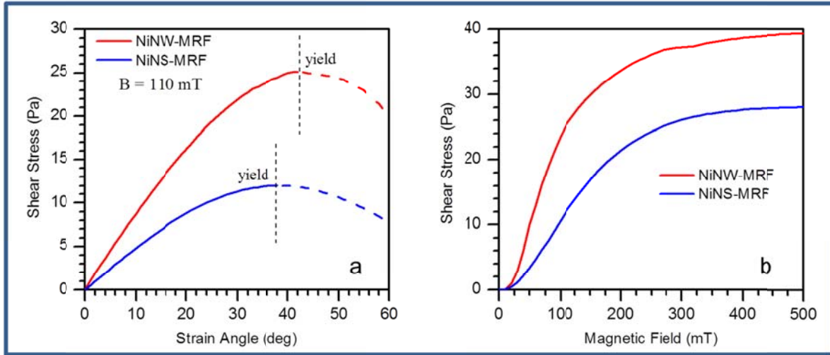
Figure 5. Calculated shear stress under an applied magnetic field. (a) Stress-strain curves of the 3 vol% NiNW-MRF and 3 vol% NiNS-MRF under an applied magnetic field B = 110 mT. NiNW-MRF yields at \theta = 43^\circ and NiNS-MRF yields at \theta = 38^\circ , beyond which the stress-strain curves beyond yield are indicated by dashed lines since flow can begin and the model becomes inappropriate. (b) Yield stress of 3 vol% NiNWs and 3 vol% NiNSs under varying applied magnetic field \mathbf{B} .
