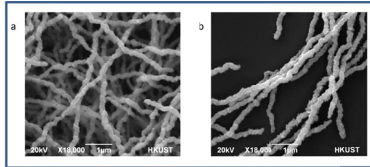
Figure 1. The SEM images of NiNWs (a) without and (b) under a magnetic field.
