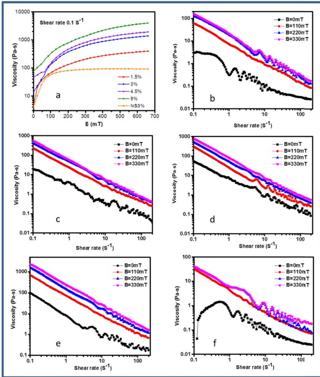
Figure 3. (a) Characterisation of changes in viscosity with varying magnetic fields. The orange colour represents NiNS-MRF, while the remainder are NiNW-MRF samples. The viscosity test of (b) 1.5 vol%, (c) 3 vol%, (d) 4.5 vol%, (e) 9 vol% NiNW-MRF samples and (f) 3 vol% NiNS-MRF with varying shear rate at constant applied magnetic field.
