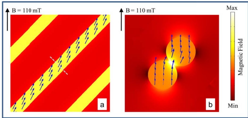
Figure 6. Calculated cross-section of magnetic fields at yield point for (a) NiNWs and (b) NiNSs under applied magnetic field B = 110 \text{ mT} . The direction of the applied magnetic field is indicated by the black arrows. The gray dashed line indicates the gap between neighbouring NiNWs. The blue vectors are the magnetisation field \mathbf{M} of the particles.
