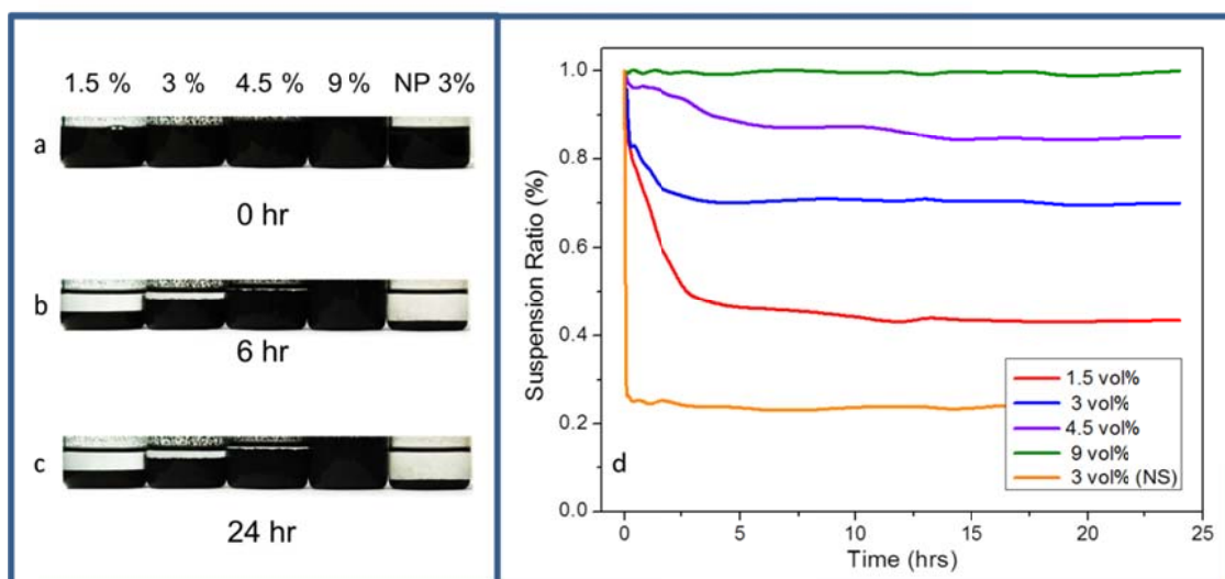
Figure 4. Photos of MRF samples during sedimentation (a) at the beginning, (b) 6 hrs later, and (c) 24 hrs later. (d) Graph of suspension ratio changes within 24 hrs.
