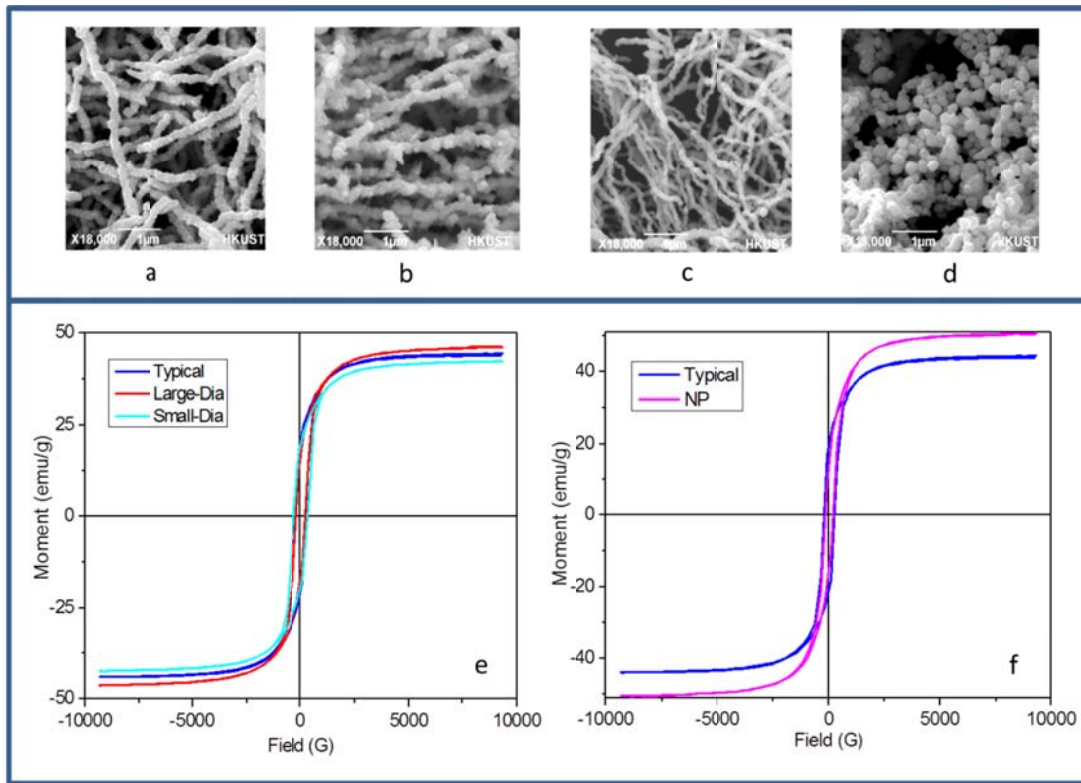
Figure 2. SEM images with the same magnification of (a) typical synthesized NiNWs, (b) NiNWs synthesized at 70 °C, (c) NiNWs synthesized at 140 °C, and (d) NiNSs. Hysteretic loops at room temperature of (e) typical NiNWs compared to other size NiNWs and (f) NiNWs compared to NiNSs.
