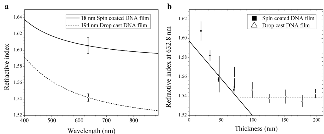
Figure 3. (a) Comparison of the refractive indices between surfactant-free DNA films with thicknesses of 18 nm made by spin coating and 194 nm made by drop casting in the visible spectral range. (b) Refractive index as a function of the thickness of surfactant-free DNA films at \lambda = 632.8 nm. Error bars in (a) and (b) are the greater of standard errors in the ellipsometric fit and standard errors in the mean (SEM) of the measurements.
