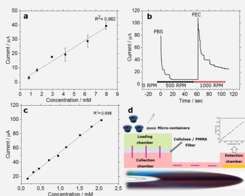
Fig.2 a) Calibration curve for model electrochemical analyte: ferrocyanide, b) Real-time detection of analytes using the disc shown in Fig. 1a: Initially PBS is loaded into the loading chamber and was spinned at 500 RPM to wet the electrodes and to get background current, followed by addition of 100 \mu l of ferrocyanide in the loading chamber and spin at 1000 RPM hence moving the analyte from loading chamber to detection chamber, c) Calibration curve for paracetamol, d) cartoon depicting the cross section view of the microfluidic disc with cellulose filters
