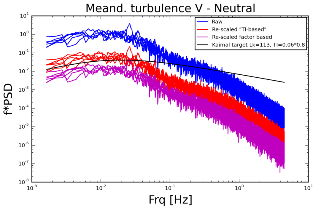
Figure C.2: Comparison of the used neutral conventional turbulence spectra with the Kaimal ref. spectrum ( ti=6\% ). The “raw” box spectrum is plotted together with rescaled turbulence using respectively 1) turbulence intensity based and 2) “factor” based scaling. Top: u-component; Bottom: v-component.
