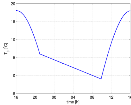
Figure 26: Temporal variation of ground temperature.
