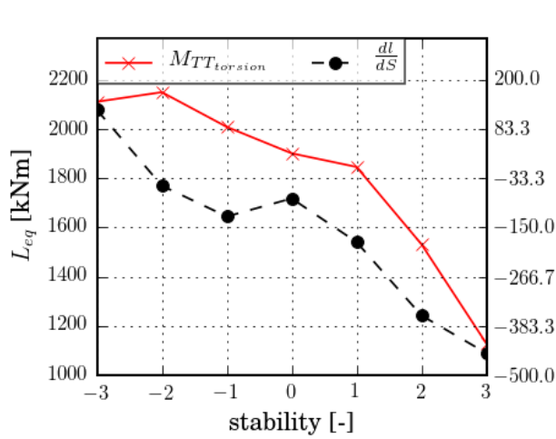
Figure 90: The 5D 8m/s case. (left) Load response function, M_{TT_{torsion}} (red), and its derivative, dI/dS (black), for the tower top torsion moment as function of the stability identifier; (right) Load response pdf and cdf for the blade root flap moment.
