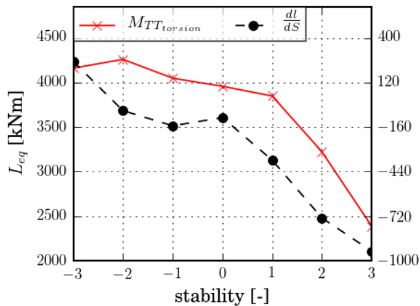
Figure 91: The 5D 14m/s case. (left) Load response function, M_{TT_{torsion}} (red), and its derivative, dI/dS (black), for the tower top torsion moment as function of the stability identifier; (right) Load response pdf and cdf for the blade root flap moment.
