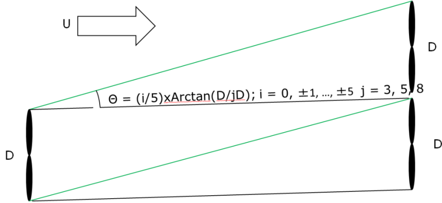
Figure 83: Generic WF layout and the defined set of inflow cases.
