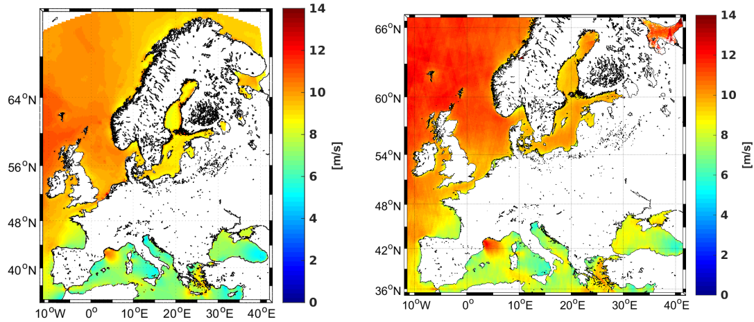
Figure 4. Mean wind speed at 100 m from ASCAT (left) and the combination of Envisat-ASAR and Sentinel-1 (right).
