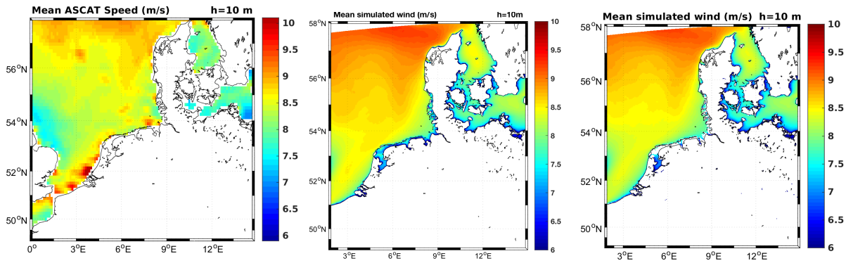
Figure 5. Mean wind speed at 10 m above the ocean surface from ASCAT (left) and WRF using the MYNN (middle) and YSU (right) PBL schemes, for 2015.
