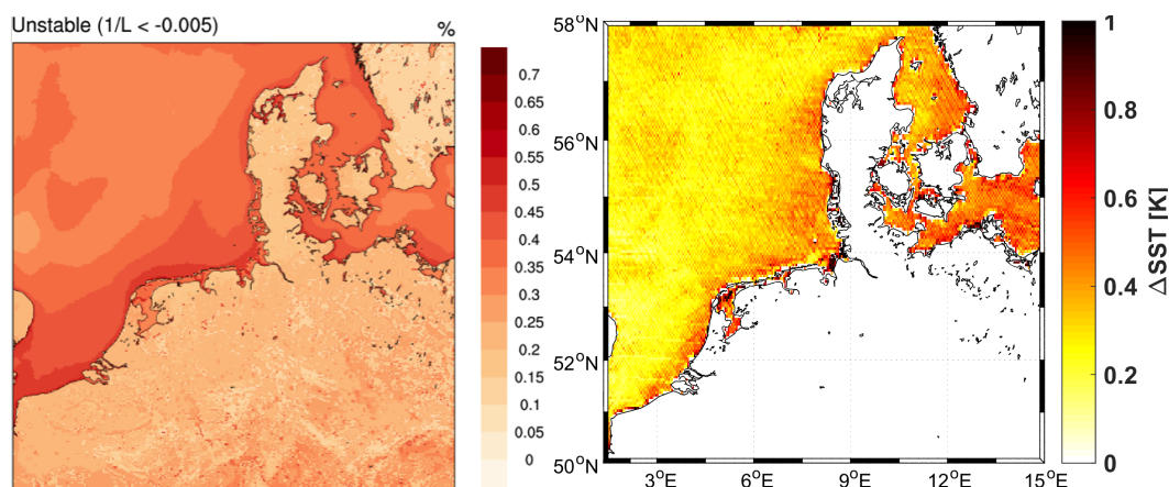
Figure 6. Fraction of unstable conditions over the North Sea during 2015 as simulated by WRF during the sensitivity experiments (left). Mean of the sea surface temperature maximum diurnal variability from 2006 to 2012 (right).
