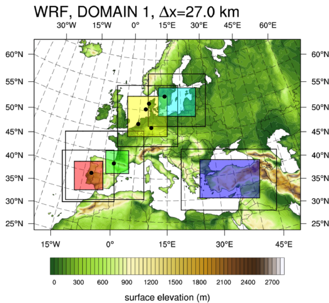
Figure 1. The WRF outer domain over Europe with the 5 nested, higher resolution domains shaded in different colours: NE (turquoise), NW (yellow), PE (red), SW (green) and SE (purple). The black dots represent sites of experimental measurement campaigns during the NEWA project.
