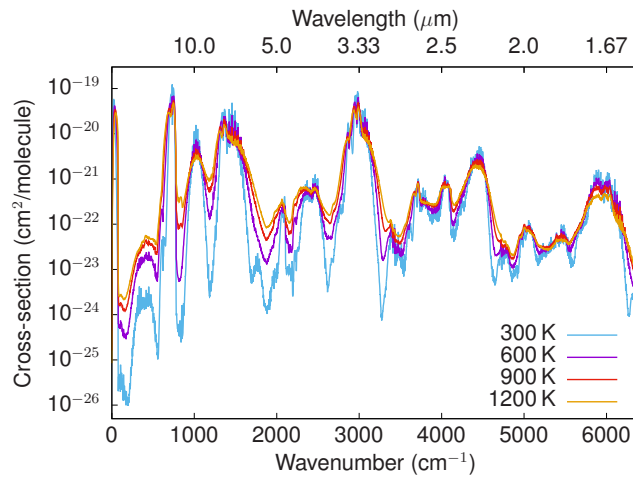
Figure 5. The OYT-35 line list temperature dependence: the spectrum becomes increasingly flat as the temperature is raised.
