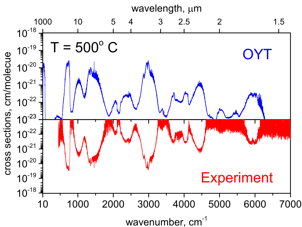
Figure 8. OYT absorption cross-sections simulated at 500 °C compared with the newly measured IR spectrum. Noise between 4700 – 7000 \text{cm}^{-1} is due to the light source and poor MCT detector sensitivity in that region.
