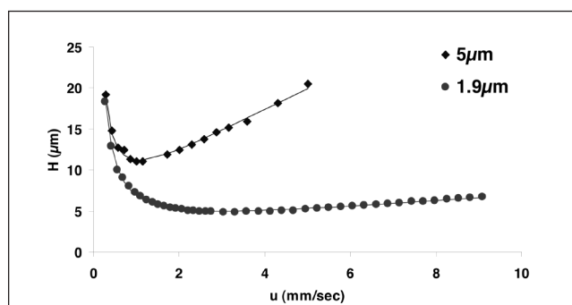
Figure 3. Effect of particle size on the chromatographic performance of Hypersil GOLD support. Solute: Butylparaben. Van Deemter curves H = f(u) for: \blacktriangle = 150 \times 4.6 mm, 5 \mu\text{m} , and \bullet = 50 \times 2.1 mm, 1.9 \mu\text{m} .
