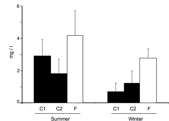
Fig. 8: Total free sulfides (TFS) in mg/l (mean \pm SE) in sediment, at each control (C1 and C2) and fish farm location (F), during summer and winter season.
