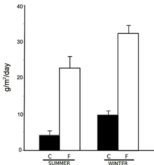
Fig. 2: Sedimentation rates of total organic matter (mean ± SE) estimated using sediment traps at control (C) and farm (F) locations, during summer and winter seasons.
