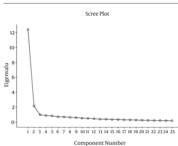
Figure 1. The Scree Plot of a 25-Item Exam Preparation Scale
