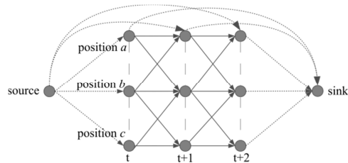
Fig. 2. Graph construction
