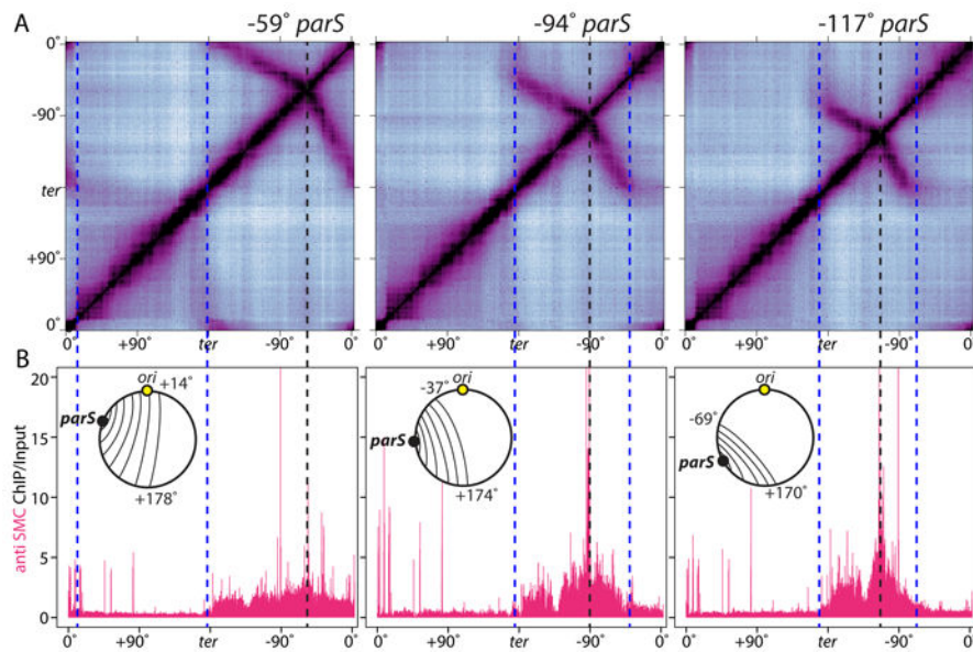
Figure 2. Condensin is specifically enriched along juxtaposed DNA
