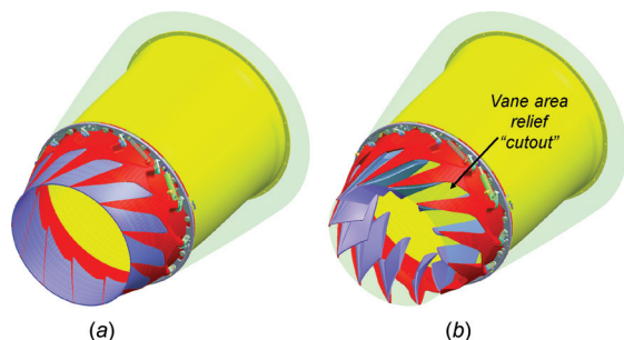
Fig. 2 EAB CAD model in two configurations. Translucent green region shows allowable zone boundary. Vane area cutout feature controls effective exit area: (a) stowed and (b) fully deployed (100 deg).
