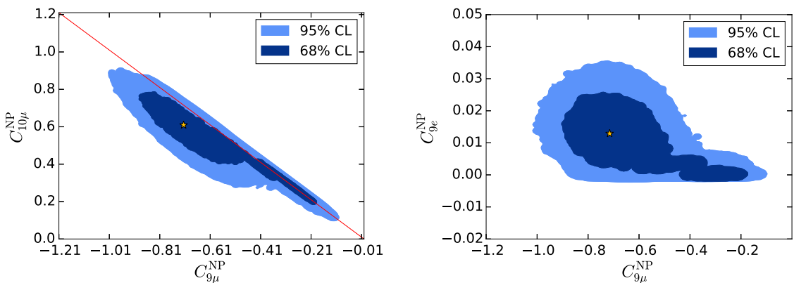
Figure 3. Allowed regions at 68% and 95% CL from the global fit for the Wilson coefficients of b \rightarrow s \ell^+ \ell^- transitions. The best fit point is illustrated with a star. The red line on the left plot illustrates the correlation C_{9\mu}^{\text{NP}} = -C_{10\mu}^{\text{NP}} .
