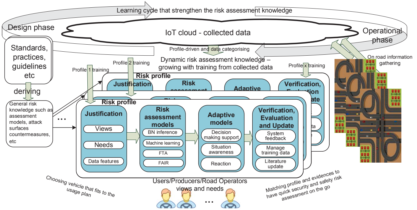
Figure 1: Profile-driven dynamic risk management framework
