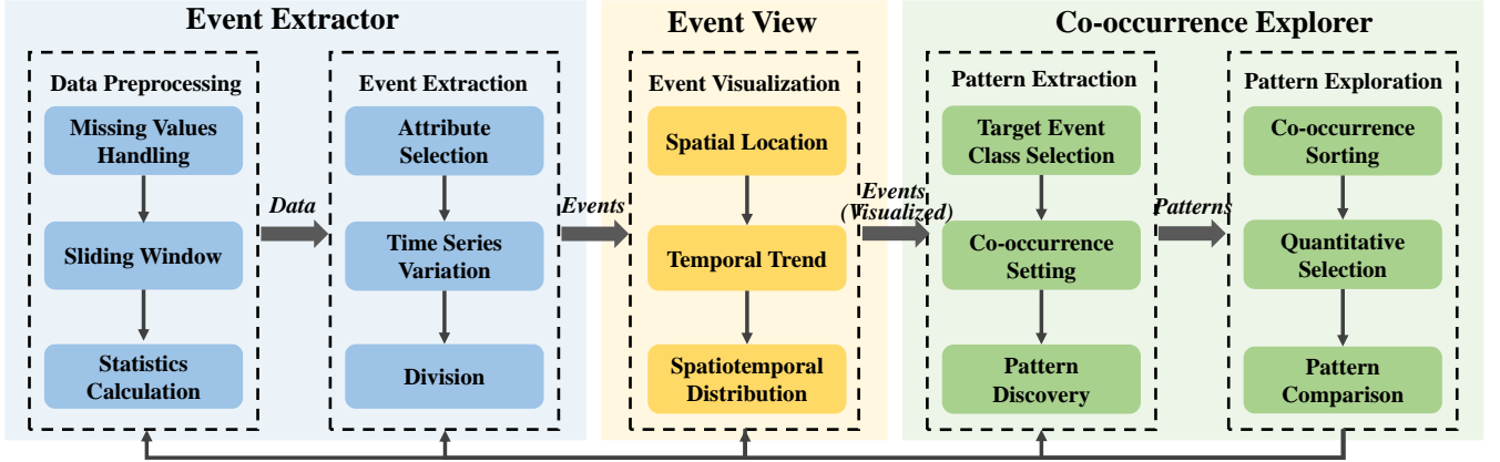
Fig. 4. Analytical Pipeline. The pipeline enables drilling down from original data to pattern discovery. It is supported by three interactive visual components marked with different background colors.
