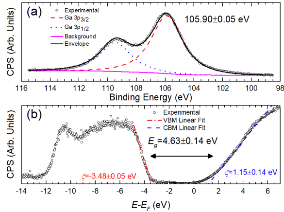
Fig. 1 – This figure shows (a) the Ga 3p core levels, and (b) the valence band obtained by XPS and the conduction band edge obtained by IPES for the 30nm \text{Ga}_2\text{O}_3 sample.
