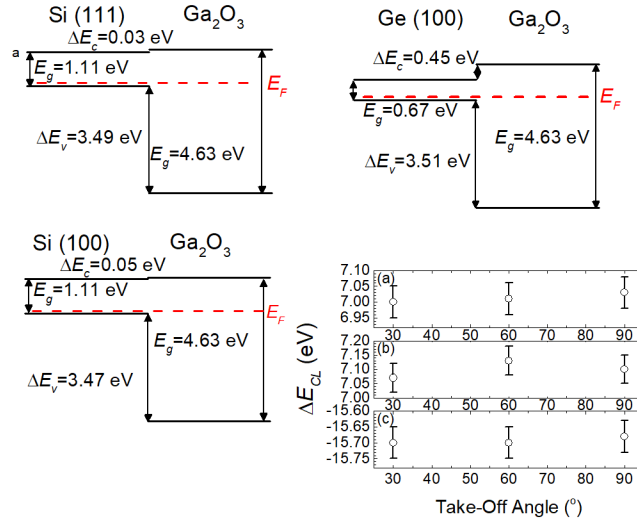
Fig. 4 – A schematic band alignment diagrams showing the XPS determined band alignments for ALD-grown Ga 2 O 3 on a variety of common semiconductor substrates.
