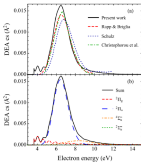
FIGURE 6.28: DEA Cross-section of O_2 . Credit: [92].
