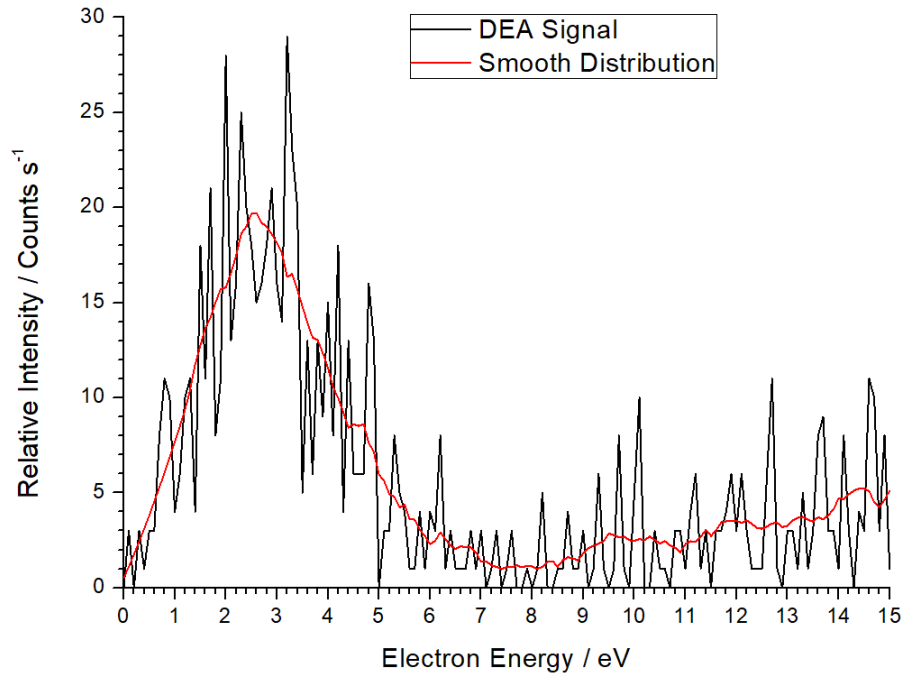
FIGURE 6.29: DEA signal representing the attachment ( O^- ions) probability of fast O_2 . Energy filter = 25 eV.
