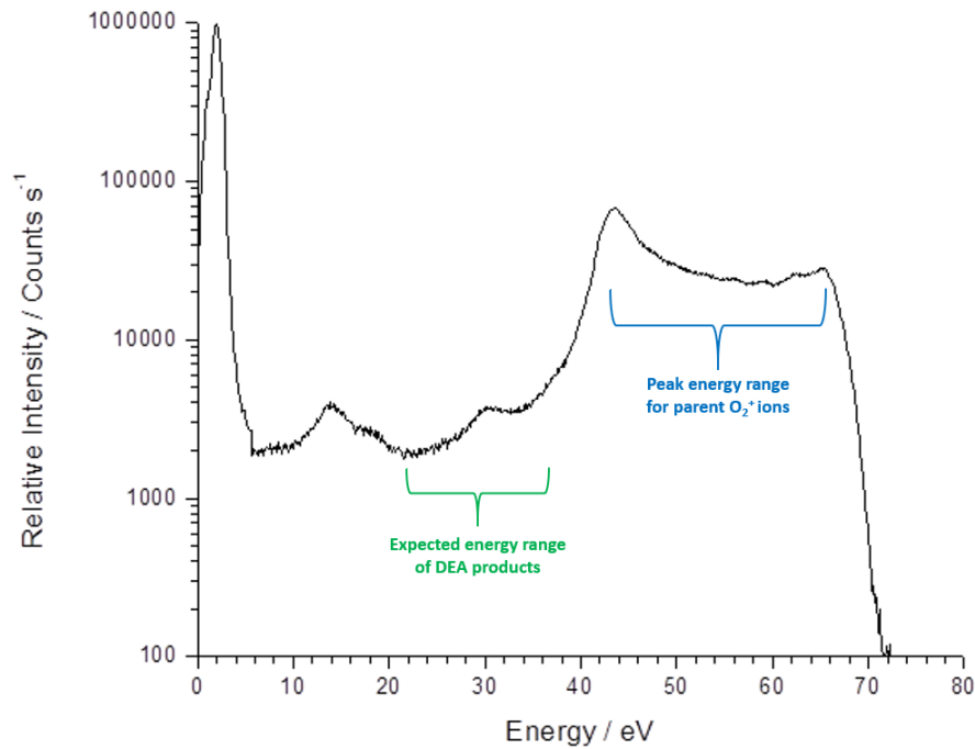
FIGURE 6.25: Extended IED of O_2^+ is representative of capacitive mode.
