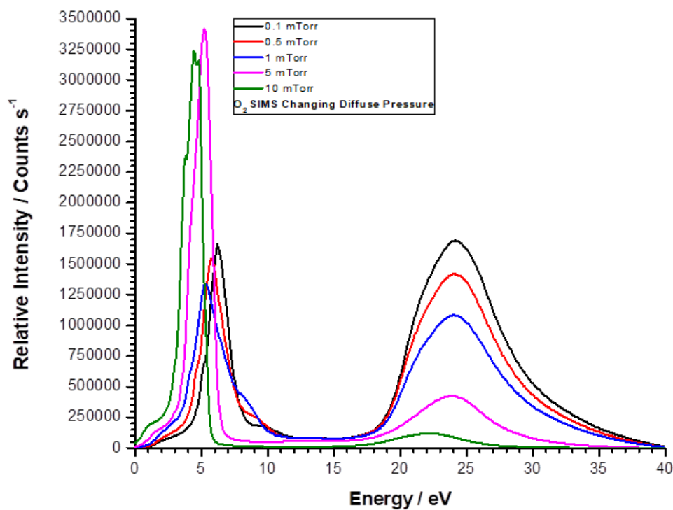
FIGURE 6.22: O_2^+ (350 W) energy distribution with changing neutralization pressure in pure SIMS mode.
