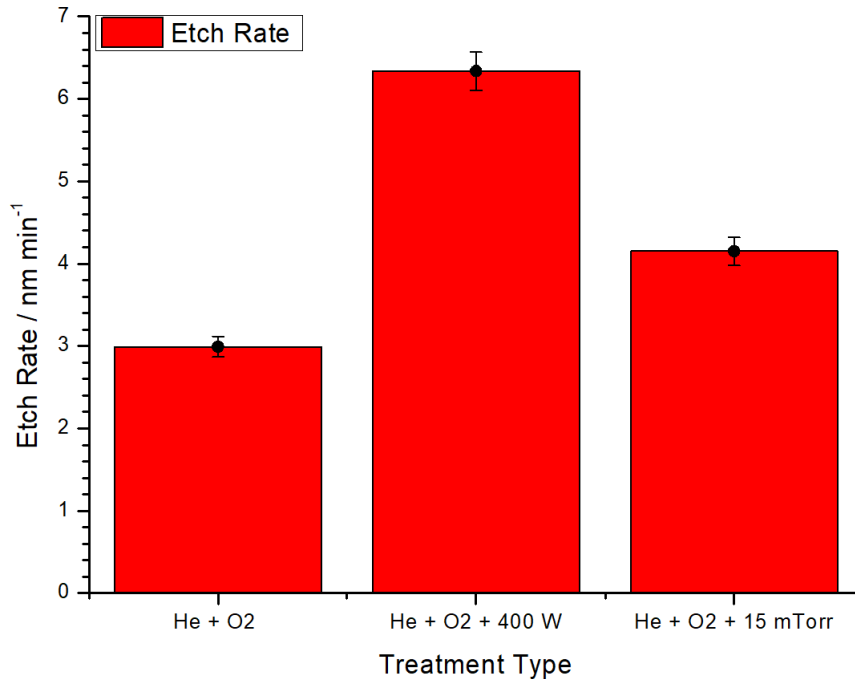
FIGURE 7.26: Etch rates of FCP with a carbon neutralizer.
