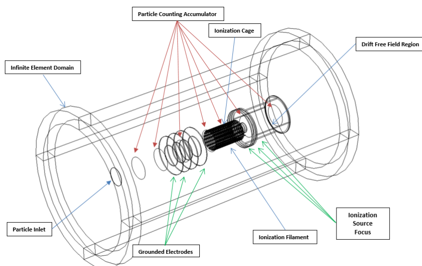
FIGURE 5.6: Annotated schematic of the EQP flight path.
