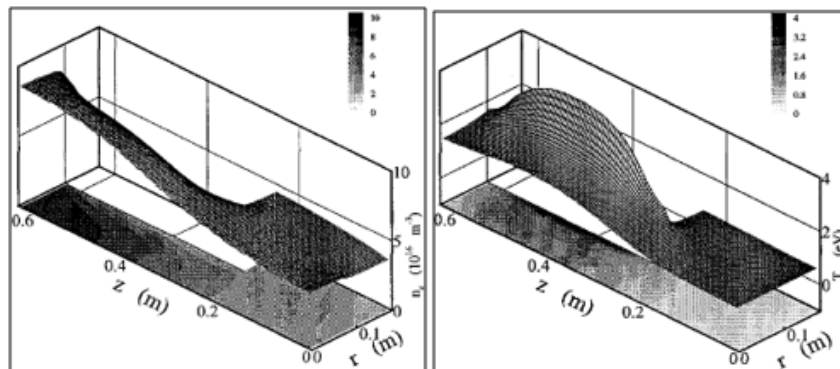
FIGURE 4.29: Left to right , electron density and temperature Credit: [69]
