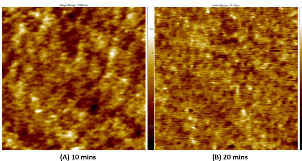
FIGURE 7.23: AFM image of the FCP surface at (A) 10 minute: \Delta z = 2.95 nm and (B) 20 minute: \Delta z = 0.73 nm.
