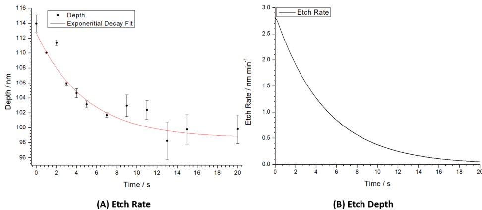
FIGURE 7.10: Evolution of HCP etch depth and etch rate with time in a He + O 2 30 mTorr 200 W plasma. Exposure was with just UV photons, diffuse neutrals and energetic neutrals from gas phase charge-exchange.
