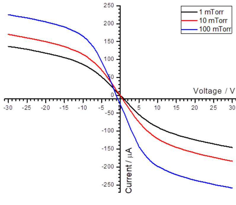
FIGURE 4.7: Double probe I-V curve as a function of pressure.
