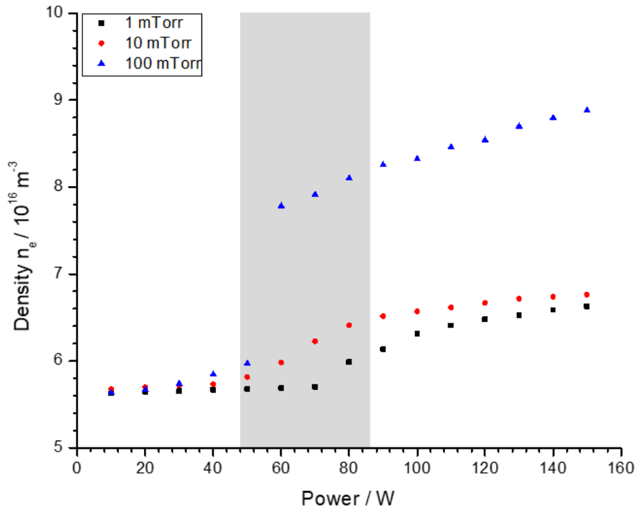
FIGURE 4.4: Electron density in Ar varied with power. The region of transition into H-mode is highlighted in grey.
