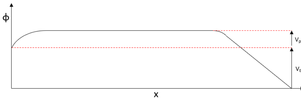
FIGURE 6.3: Schematic of biased plasma potential structure. x axis is distance. V_p and V_b represent the plasma potential and plasma bias respectively
