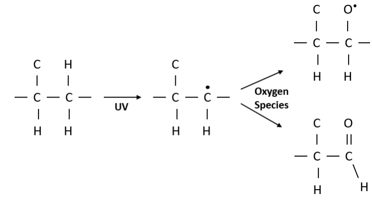
FIGURE 7.11: Illustration of UV causing photochemistry on a HCP polymer. UV photons cause dehydrogenation which are then occupied by oxygen species in single cross-link and double bonds for surface hardening.
