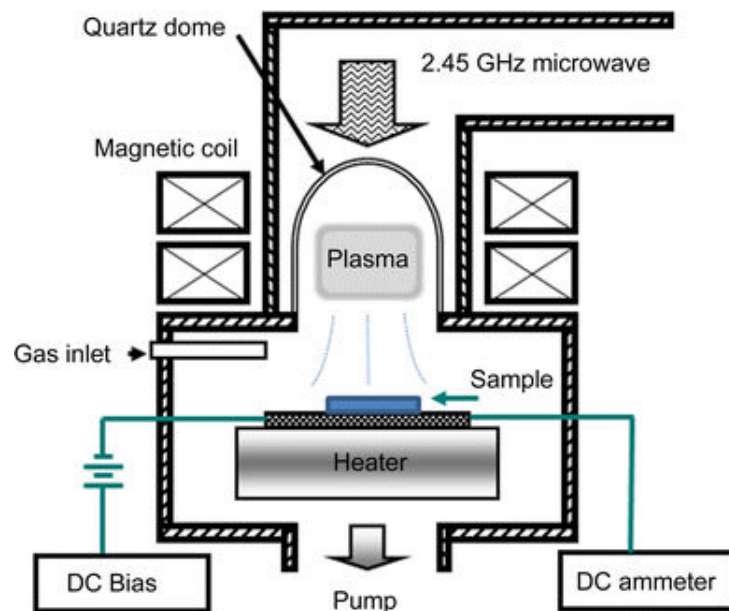
FIGURE 1.6: Schematic of an ECR plasma setup. Resonance occurs in specific regions of the plasma thus requiring restrictions on wafer and reactor size. Credit: Tseng, 2008 [10]
