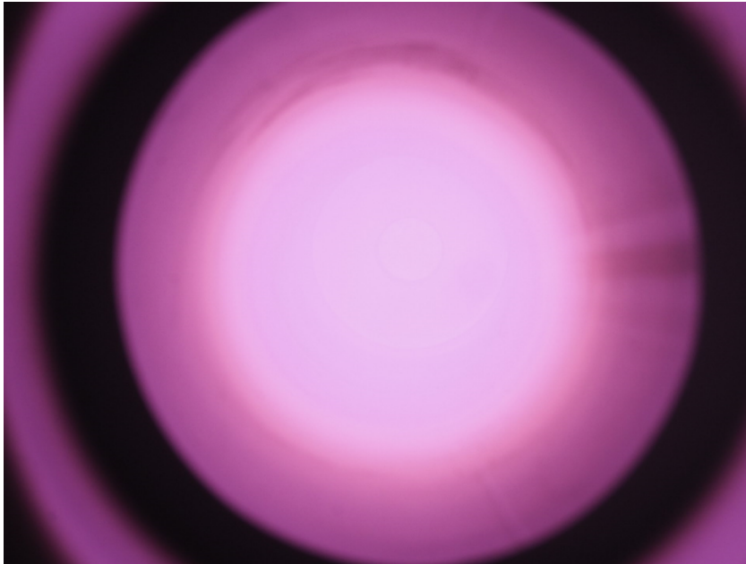
FIGURE 4.36: Picture of the plasma (250 W, 1 mTorr) taken above from an optical window.
