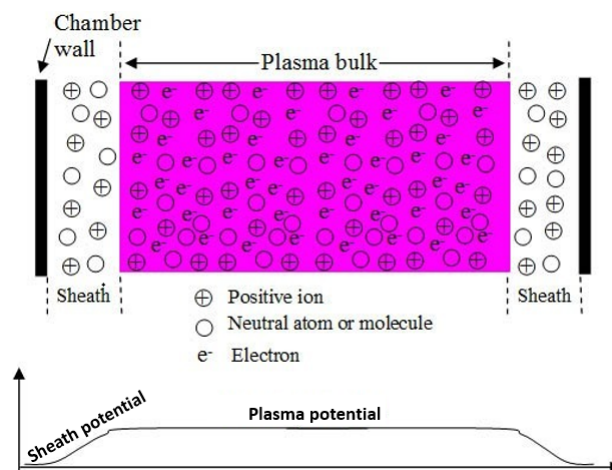
FIGURE 1.2: Variation of charge density and potential from the bulk of the plasma to the wall. Credit: Pie Scientific
