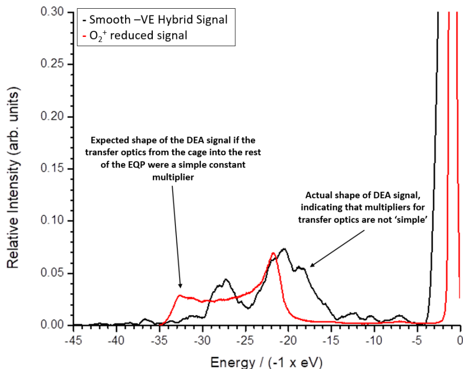
FIGURE 6.33: DEA signal superimposed on to the Energy of parent ions with reduced horizontal and vertical scale.
