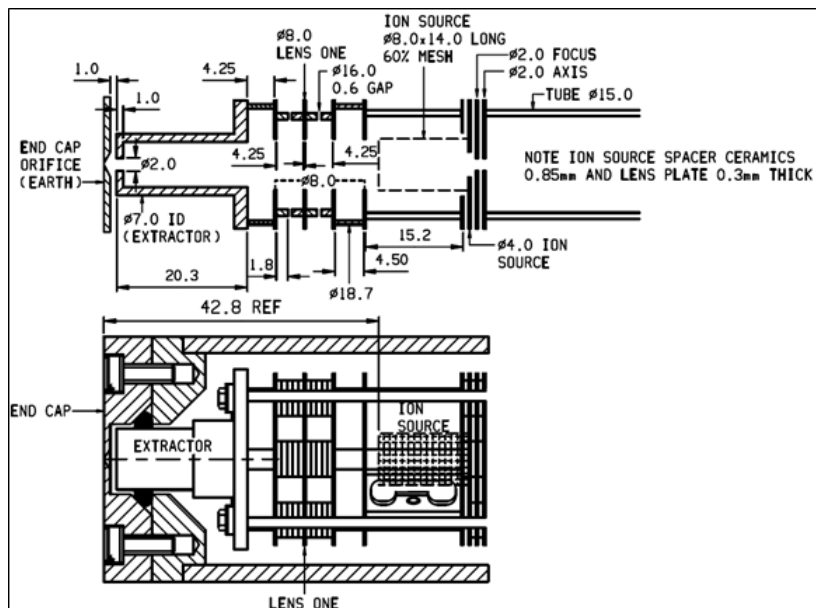
FIGURE A.3: Hiden EQP Schematic 2. Credit: Hiden Analytical
