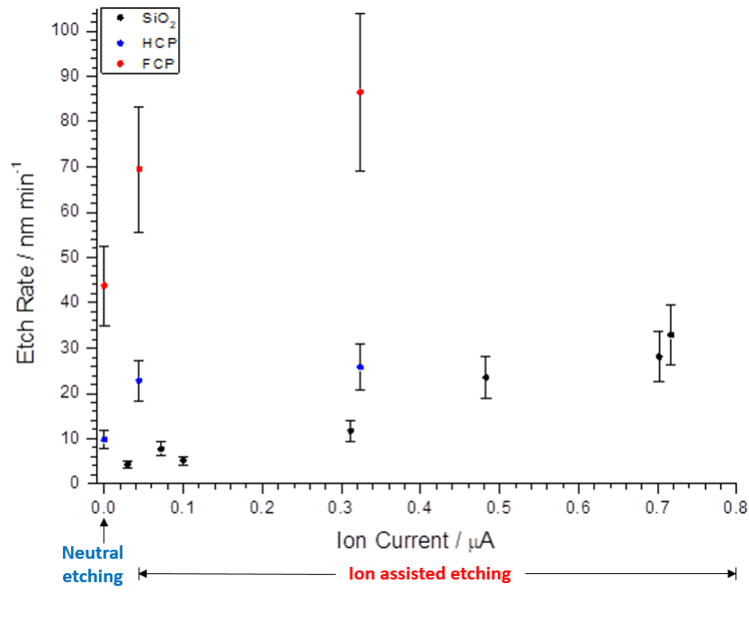
FIGURE 7.5: Etch rate varying with ion current in a single extractor arrangement (gas phase) with a 250 W & 5 mTorr plasma. The gas mixture was 10 SCCM O 2 + 1 SCCM SF 6 .
