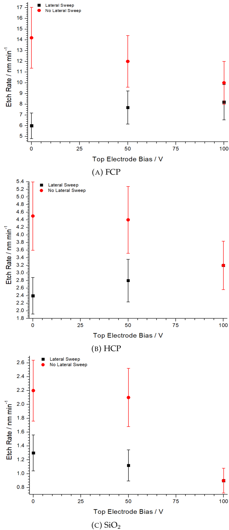
FIGURE 7.7: Plasma conditions are identical to Figure 7.6 . The decreasing etch rate ( red trace ) is the result of charge build-up due to increasing flux of ions to the surface.
