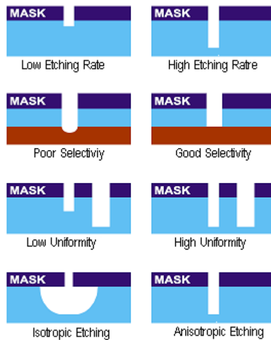
FIGURE 1.8: Visualization of common etching parameters. Credit: Adapted from O'tell, 2014
