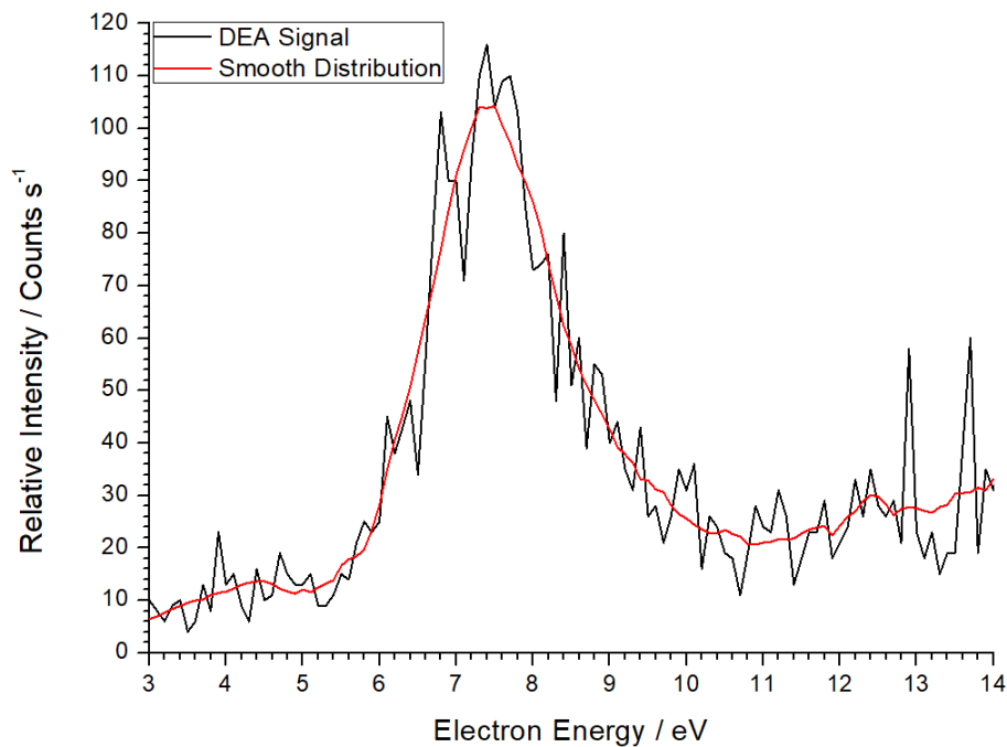
FIGURE 6.27: DEA signal representing the attachment ( O^- ions) probability of cold O_2 . Energy filter = 2 eV.
