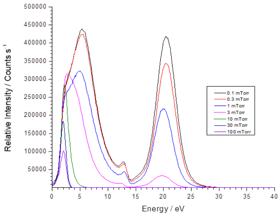
FIGURE 6.7: SIMS scan of \text{Ar}^+ 250 W with pressure. The increase of the pressure results in the suppression of the energy distribution function.
