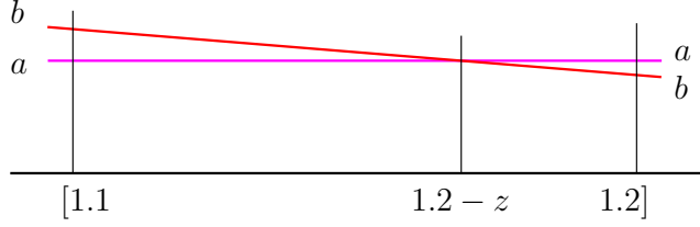
Fig. 2. This figure shows how -\dot{p}_2 is computed on the interval [1.1, 1.2] for the location l_R . The function is given by the upper envelope of the two functions: it agrees with the quality of a on the interval [1.2 - z, 1.2] and with the quality of b on the interval [1.1, 1.2 - z] .
