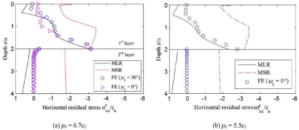
Figure 8 Comparison between FE calculated residual stress field and critical residual stress fields when \phi_1 = 30^\circ , \phi_2 = \psi_2 = 0^\circ , E_1/E_2 = 3
