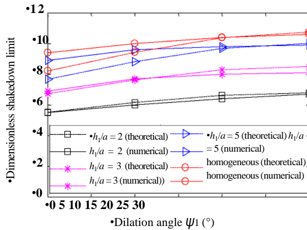
•Figure 11 Comparison of theoretical and numerical shakedown limits in two-layered pavements with varying first layer thickness when \theta_1 = 30^\circ , \theta_2 = \psi_2 = 0^\circ , E_1/E_2 = 3 , c_1/c_2 = 1
