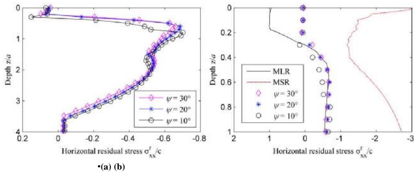
•Figure 4 Influence of dilation angle on horizontal residual stress field when \phi = 30^\circ, p_0 = 10.6c
