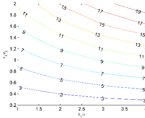
• Figure 12 Contour of dimensionless shakedown limits as an example chart for the thickness design of a two-layered pavement when \varphi_1 = 44^\circ , \psi_1 = 25^\circ , \varphi_2 = \psi_2 = 0 , E_1/E_2 = 3
