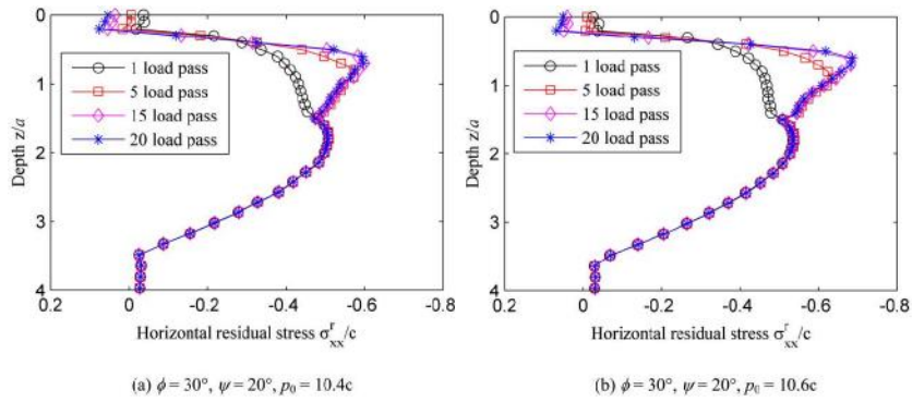
•Figure 3 Development of horizontal residual stress field
