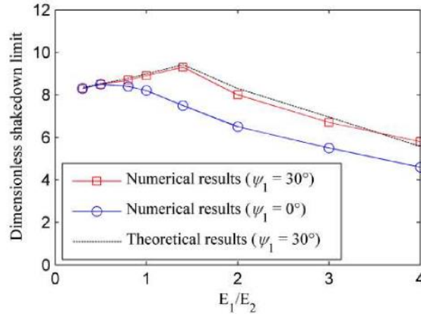
•Figure 7 Comparison of numerical and theoretical shakedown limits for layered pavements when \varphi_1 = 30^\circ , \varphi_2 = 0^\circ , c_1/c_2 = 1
