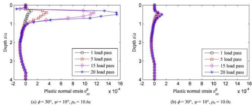
•Figure 5 Development of plastic normal strains
