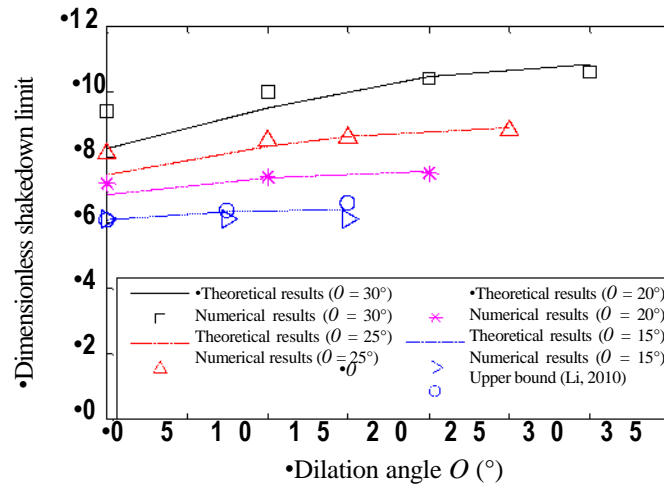
Figure 9 Comparison of theoretical and numerical shakedown limits for single layered pavements
