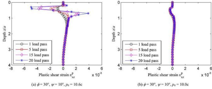
•Figure 6 Development of plastic shear strains
