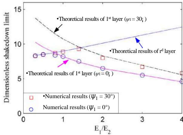
•Figure 10 Comparison of theoretical and numerical shakedown limits with varying stiffness ratio when \theta_1 = 30^\circ , \theta_2 = \psi_2 = 0^\circ , c_1/c_2 = 1
