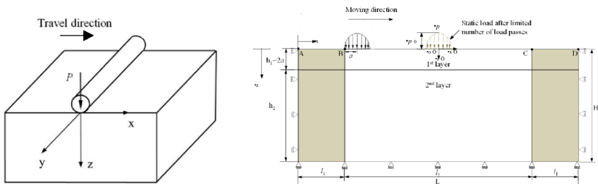
•Figure 1 Idealised pavement model Figure 2 Model sketch and boundary conditions and •2D Hertz load distribution
