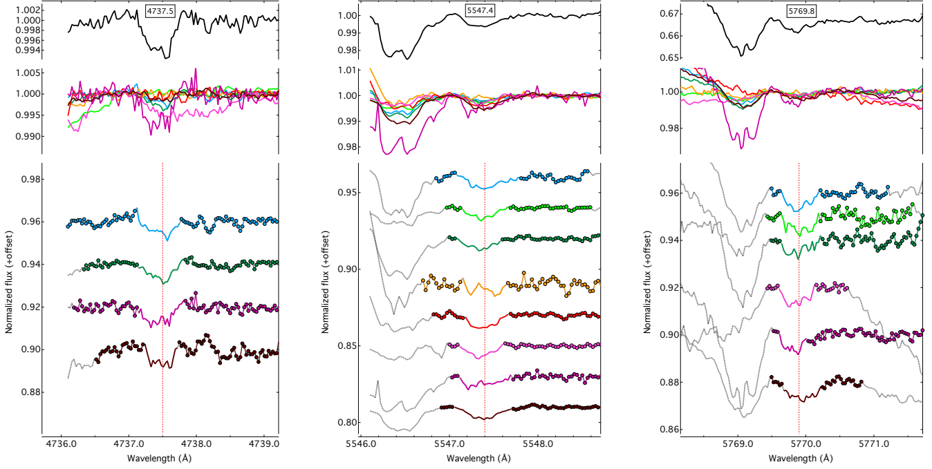
Fig. 9. Potential new detection of weak C_2 -DIBs at 4737.5, 5547.4 and 5769.8 Å (they appear toward sightlines where the other C_2 -DIBs are well-detected). The red dashed line shows the DIB location. Top graphs (black) in all three panels: extracted average normalized profile of C_2 -DIBs created from stacking three single-cloud targets: HD 23180, HD 203532 and HD 147889, shown below. Middle in all three panels: overlaid C_2 -DIB profiles at the same vertical scale for all stars. Bottom in all three panels: same C_2 -DIB vertically displaced and depth-equalized profiles. The red dashed line shows the DIB location. The wavelengths are in the interstellar rest frame. See for color coding Fig. 1.
