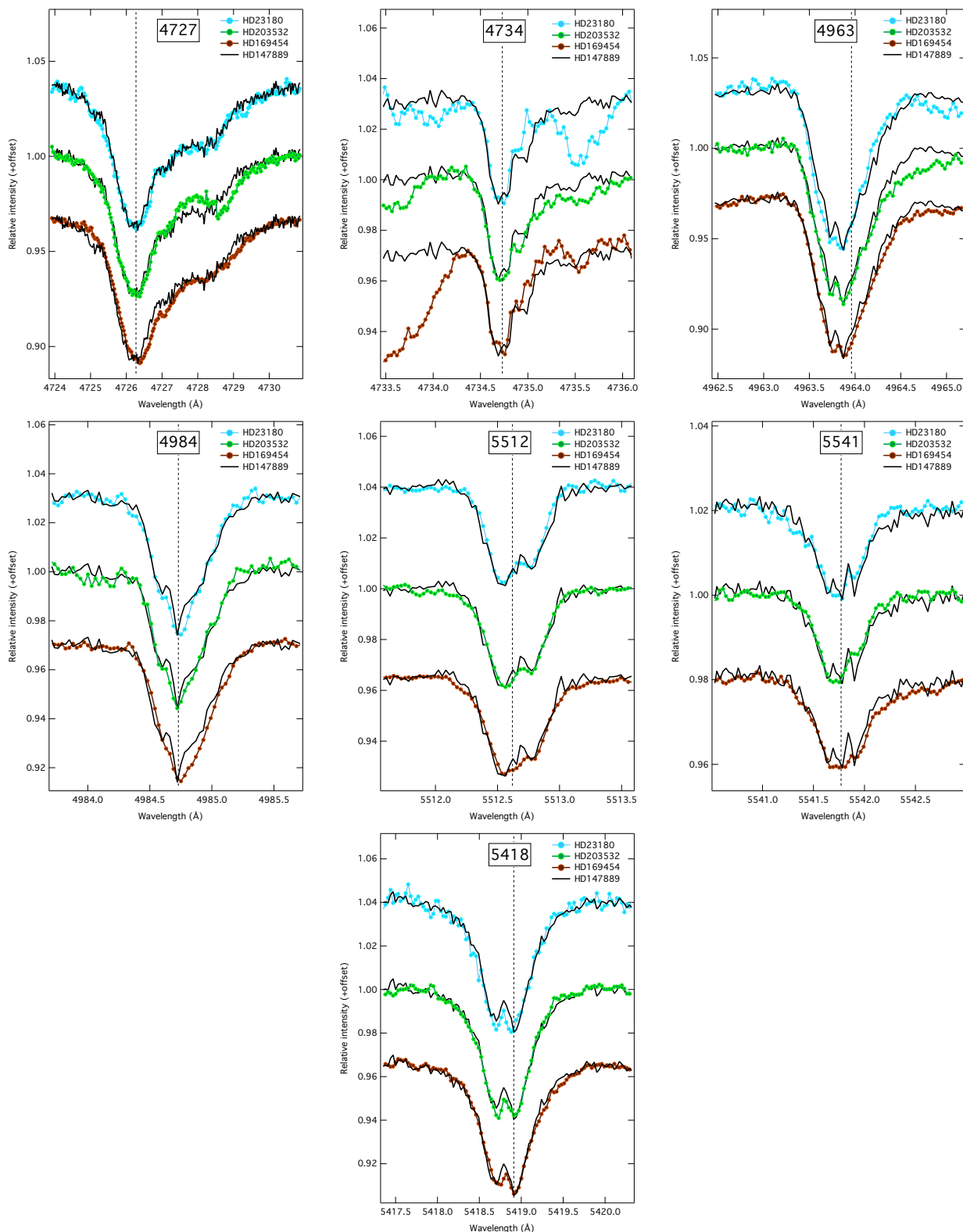
Fig. 11. Comparison between C 2 DIB profiles normalized to their central depths toward HD 23180 (blue), HD 203532 (green), HD 147889 (black) and HD 169454 (brown). The first three targets are those chosen for profile co-additions, for which results are shown in previous figures. The C 2 excitation temperatures are 20, 23 and 49K for HD 23180, HD 169454 and HD 147889 respectively (see Table 2).
