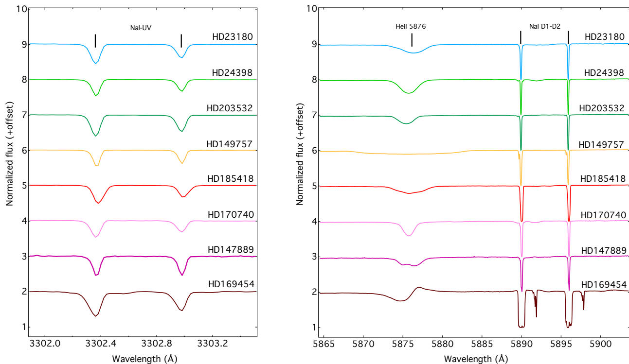
Fig. 1. Na I doublet at 3302.368/3202.987 Å (left), and Na I D1-D2 and the stellar He II (right) line are shown for the seven selected single-cloud line-of-sight (one main cloud component) and the multi-cloud target HD 169454. The Na I spectra have been shifted to their air rest wavelengths. The same velocity shift has been applied to the Na I D1-D2 lines. The applied color coding is used in all other figures as well.
