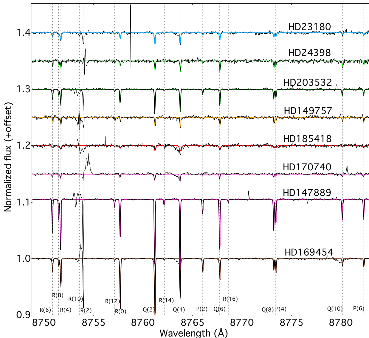
Fig. 2. Observed Phillips (2-0) C 2 bands and their best-fitting model profiles. The R 10 and R 2 lines at 8753.949 and 8753.578 Å have not been included in the fit because of the presence of a CCD artifact near these wavelengths that could not be corrected by flat-fielding. In some cases, Q(4) line is blended with a suspected DIB (or stellar line).
