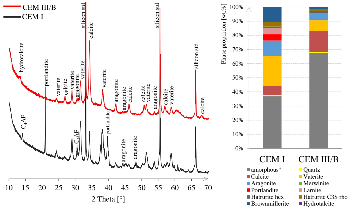
Fig. 7. XRD diffractograms with respect to the phases in: CEM I and CEM III/B carbonated powders (left), quantitative phase analysis by Rietveld method for cement paste carbonated powders after 180 days carbonation (right).
