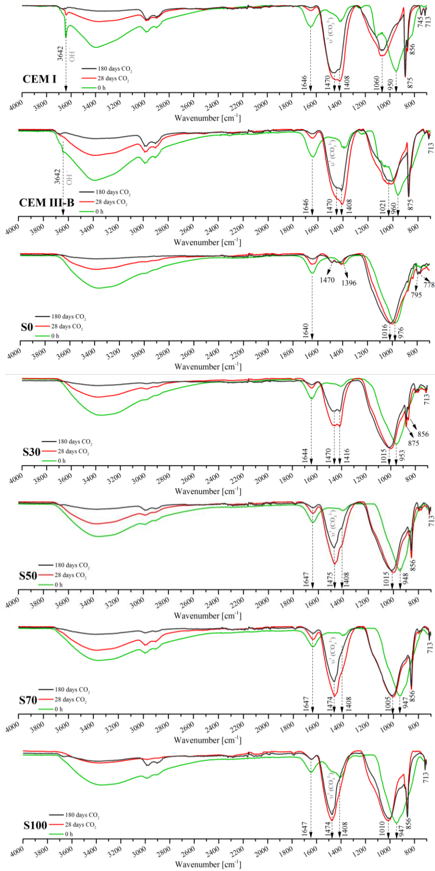
Fig. 6. FT-IR spectra of reference paste powders (samples before carbonation, 0 h, green lines), MS CO 2 curves of paste powders obtained after 28 days of continuous carbonation (red lines), MS CO 2 curves of paste powders
