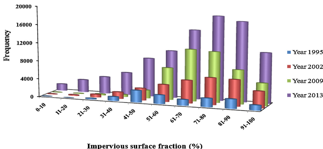
Fig. 6. Frequency histograms of impervious surface pixels in the Cixi County buffer in 1995, 2002, 2009 and 2013.
