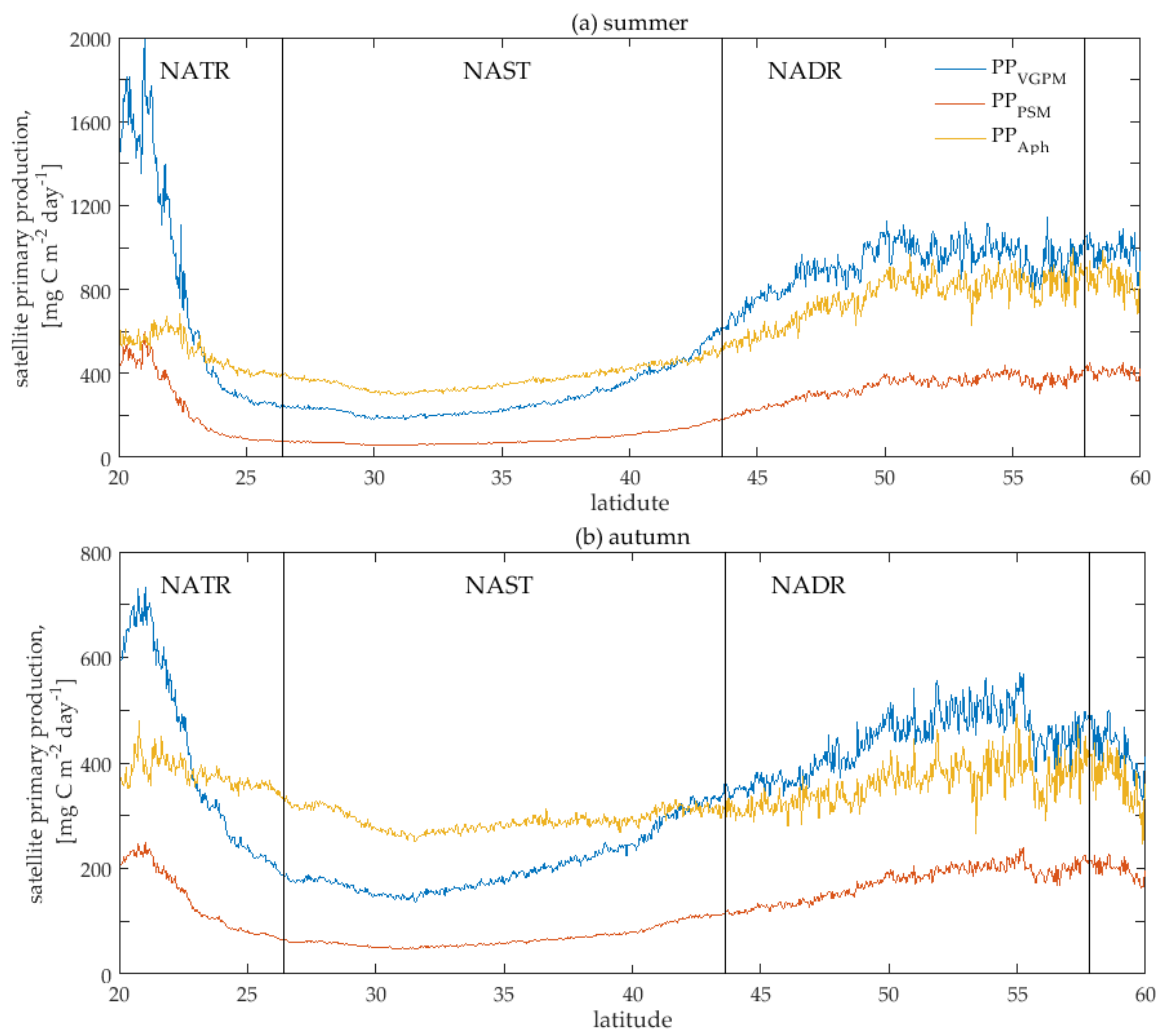
Figure 7. Spatial transects of satellite PP_{VGPM} , PP_{PSM} , and PP_{Aph} ( \text{mg C m}^{-2} \text{ day}^{-1} ) along 20^\circ\text{W} from 20^\circ\text{N} to 60^\circ\text{N} for (a) summer (June–August) and (b) autumn (September–November) using OC-CCI climatology for 1998–2011.
