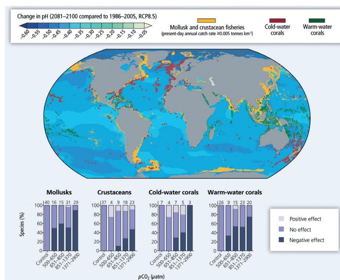
Figure 1: Vulnerability to ocean acidification. Marine mollusc and crustacean fisheries (present-day estimated annual catch rates \geq 0.005 tonnes km -2 ) and known locations of cold- and warm-water corals, depicted on a global map showing the projected distribution of ocean acidification under RCP8.5 (pH change from 1986–2005 to 2081–2100). The bottom panel compares sensitivity to ocean acidification across molluscs, crustaceans, and corals, vulnerable animal phyla with socioeconomic relevance (e.g., for coastal protection and fisheries). The number of species analysed across studies is given for each category of elevated CO 2 .
