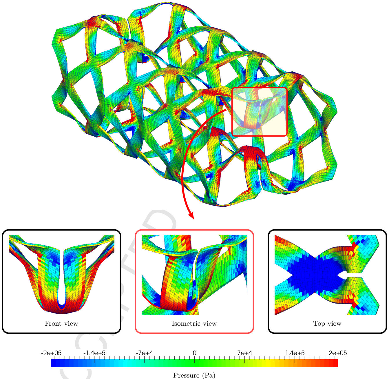
Figure 36: Stent-like structure: Snapshot of deformed shape highlighting the pressure distribution in key region using \{\mathbf{p}, \mathbf{F}, \mathbf{H}, J\} C-TOUCH scheme at time t = 500 \mu\text{s} . Results obtained with a discretisation of 6912 hexahedral elements using traction loading \mathbf{t}_b = [0, 0, -100]^T kPa. A neo-Hookean material is used with \rho = 1100 \text{ kg/m}^3 , E = 17 \text{ MPa} , \nu = 0.45 and \alpha_{\text{CFL}} = 0.3 .
