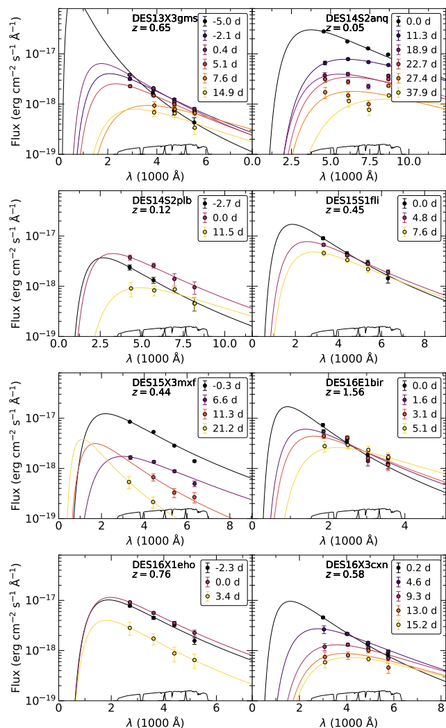
Figure 14. Example blackbody fits to eight gold sample transients. Times of individual fits are given in rest frame days since the observed peak in g band. In general blackbody matches the data well around the peak, but at later times the best fits diverge from the data.
