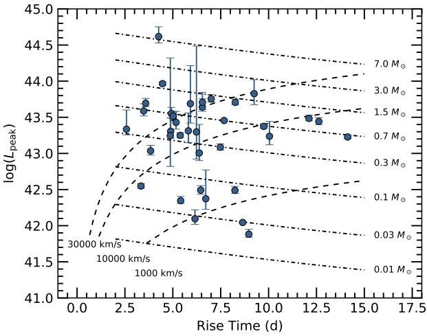
Figure 17. Bolometric luminosity based on the blackbody fits (see Table. 6) against rise time in g band for gold and silver sample events. The nearly horizontal lines correspond to required nickel mass for given luminosity and rise time. The curved lines correspond to M_{\text{Ejecta}} = M_{\text{Ni}} for a given expansion velocity assuming hydrogen and helium free ejecta ( \kappa = 0.1 \text{ cm}^2 \text{ g}^{-1} ). All points above and left from given line are unrealistic for the given velocity.
