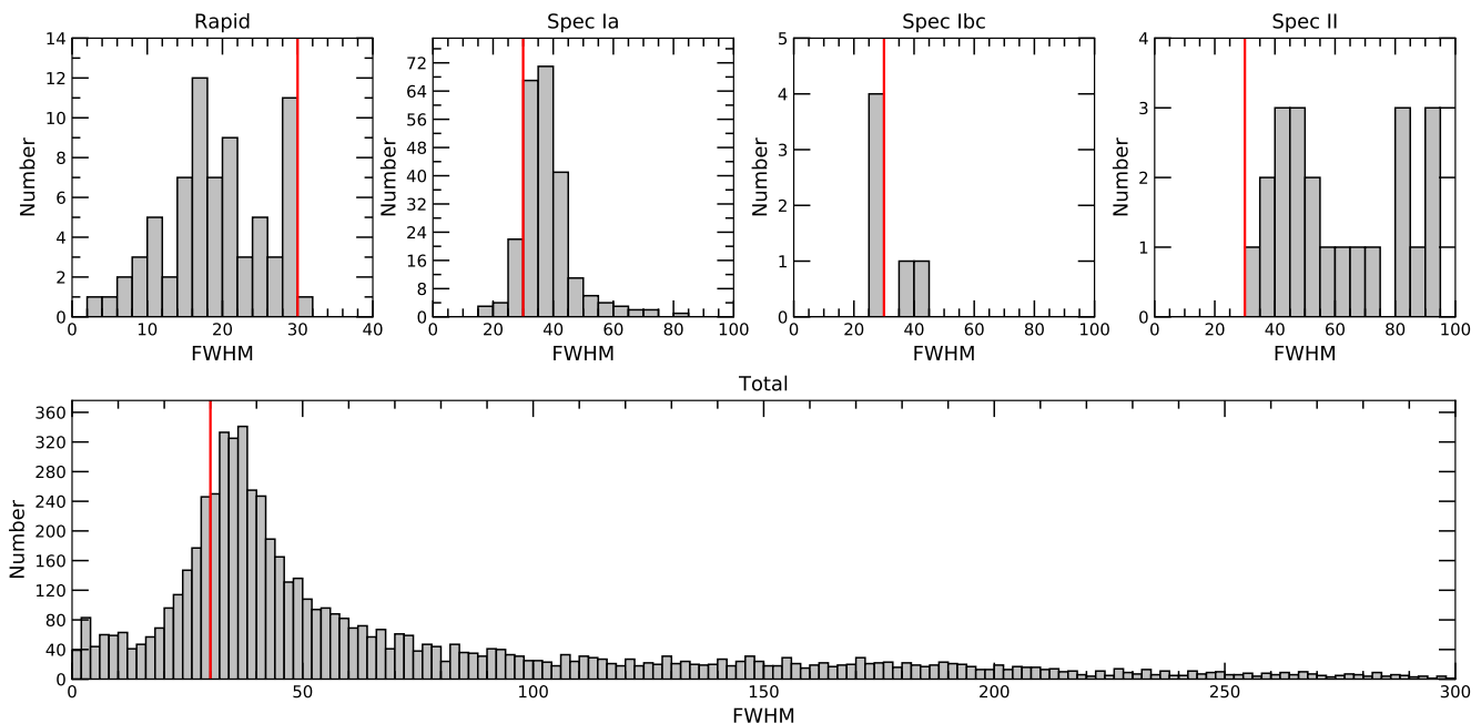
Figure 2. Mean FWHM distribution of the rapidly evolving transients in comparison with distributions of spectroscopically confirmed samples of Type Ia, Ibc and II SNe (top) and FWHM distribution of all events that passed ClassPipe (see Table 2). Red line refers to the cutoff limit of FWHM = 30 d for the rapidly evolving transients. Note that one rapid event, DES16C1cbd, has FWHM > 30 d. This event was found as part of different analysis and was included in our sample due to apparent similarity of the light curve evolution with the rest of our sample. All events found above FWHM = 300 d are ignored in the bottom panel.
