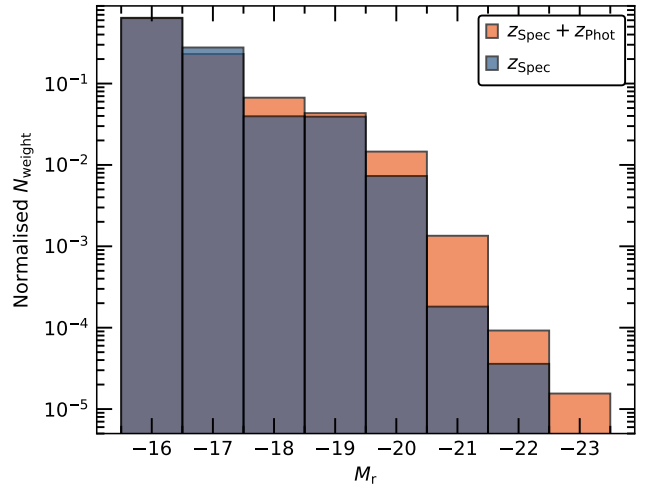
Figure 8. Normalized 1/V_{\max} luminosity distribution for 37 events with spectroscopic redshifts (Blue) and for all 63 events associated with a host galaxy including the bronze sample transients (Orange). Distributions have been normalized so that area under the curve equals unity.
