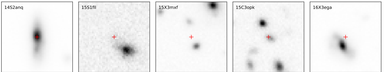
Figure 3. Explosion environments for five gold and silver sample transients. Transient explosion sites are marked with red crosses. Each square box is roughly 13.5'' on a side.
