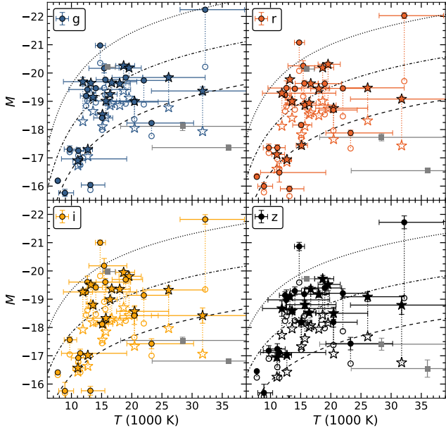
Figure 15. Peak absolute magnitude against best fitting temperature at peak. Peak magnitudes are taken from the data points closest to the peak in g band. Definition of markers is the same as in Figure 6, with the addition of grey squares referring to events for which the blackbody fits at peak were based on only two bands. Note that DES13C3bcok is ignored in this plot due to high best fitting temperature. Errors for temperatures are quoted at 1\sigma confidence. The three dashed lines correspond to absolute magnitudes in rest frame for constant radii of r = 5 \cdot 10^{14} cm (bottom), r = 10^{15} cm and r = 2 \cdot 10^{15} cm (top).
