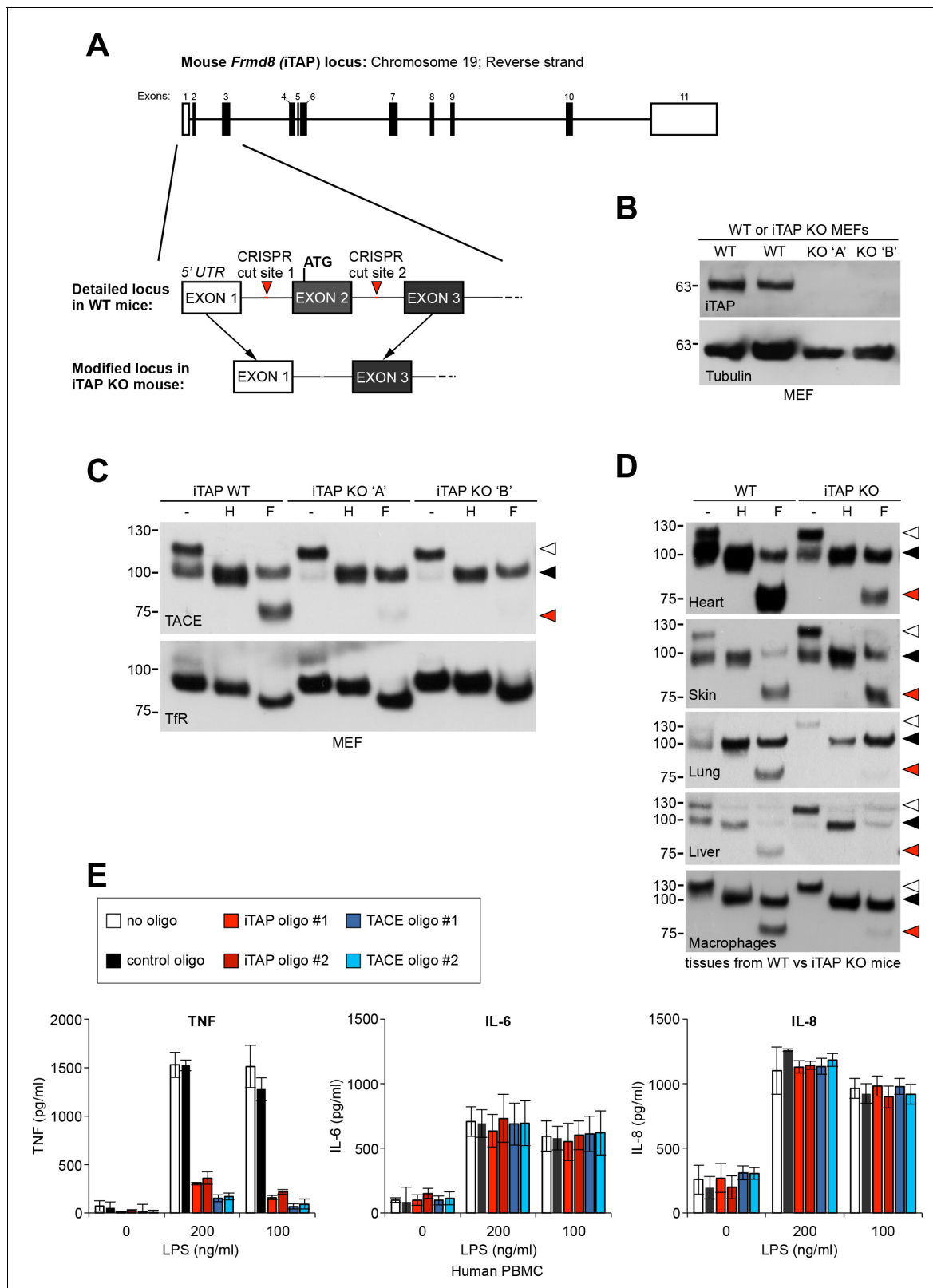
Figure 7. iTAP is essential for TACE maturation and function in primary cells and tissues from human and mouse. (A). Schematic representation of the CRISPR targeting strategy to delete mouse Frm8 (iTAP) gene using two guide RNAs flanking the first coding exon (exon 2). In the upper schematic of the Frm8 locus, open boxes indicate non-coding exons whereas filled boxes indicate coding exons (B). Mouse embryonic fibroblasts (MEFs) were isolated from WT versus two independent iTAP KO E14.5 embryo littermates. The loss of iTAP at the protein level is shown by immunoblotting. (C). Figure 7 continued on next page
