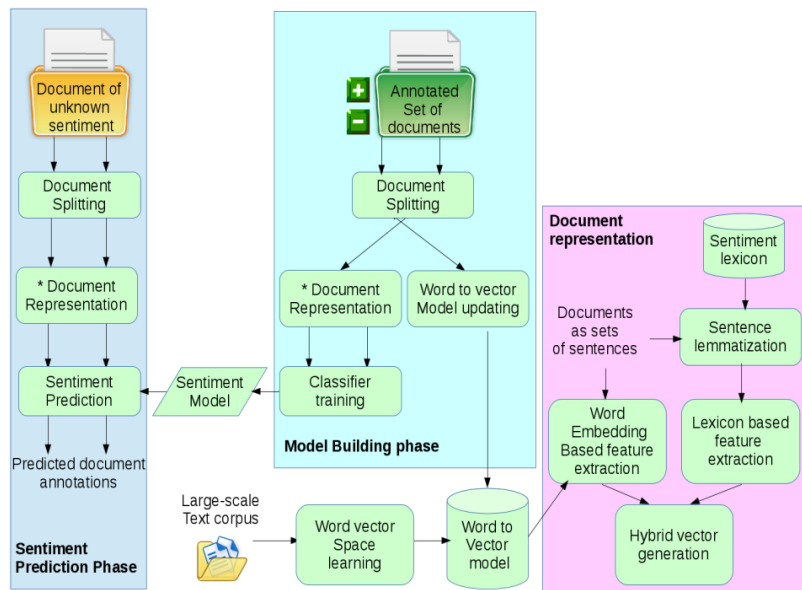
Fig 4.1. Proposed Architecture
