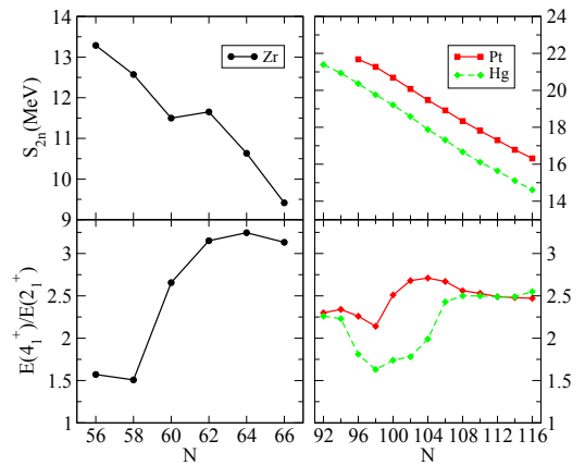
Figure 2. S_{2n} and E(4^+)/E(2^+) as a function of the neutron number, N , for Zr, Pt and Hg.
