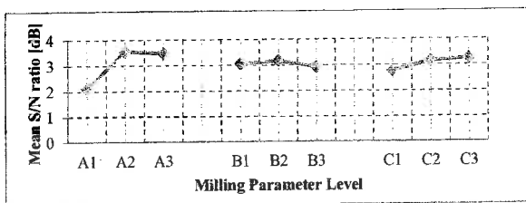
Fig. 1. Mean S/N ratio for Ra
