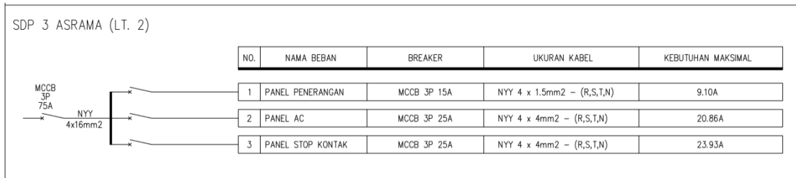
Gambar 6. SDP 3
