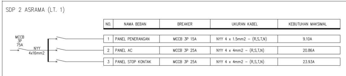
Gambar 5. SDP 2
