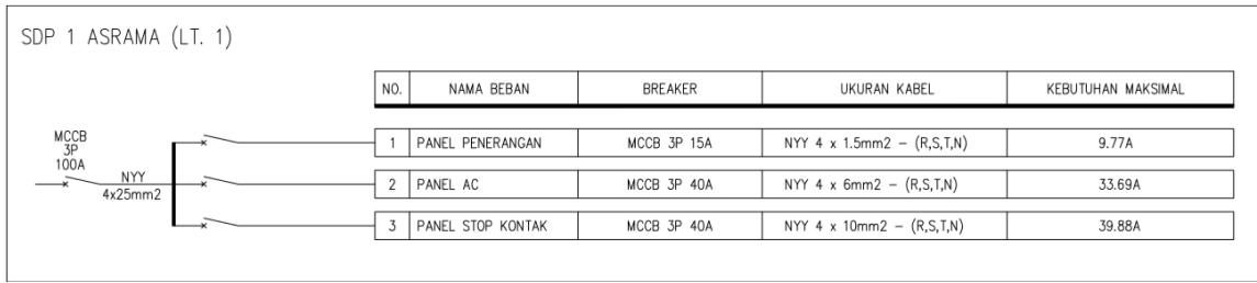
Gambar 4. SDP 1
