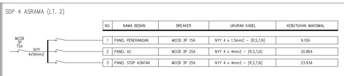
Gambar 7. SDP 4
