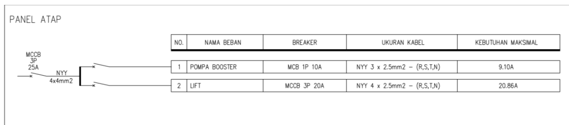
Gambar 14. Panel Atap
