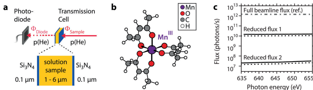
Fig. 1 (a) Schematic of the transmission-cell setup (ref. 30) for X-ray absorption spectroscopy at the L-edge of Mn III (acac) 3 in solution. (b) Molecular structure of Mn III (acac) 3 (cartoon based on the optimized structure used in ref. 15 and 23). (c) Experimental photon flux for different configurations of the undulator beamline UE52_SGM at the BESSY II synchrotron (solid: sample A; dotted: sample B) as compared to the full beamline flux (dash-dotted) from ref. 15.
