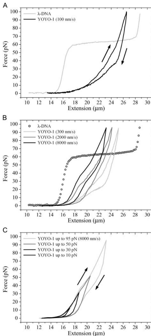
FIGURE 3 (A) YOYO-1 ( 1 \mu\text{M} ) bisintercalated \lambda -phage DNA molecule reveals hysteresis effects during extension/relaxation loop even at low stretching and relaxing velocities. (B) At increased velocities, elasticity curves are shifted to lower extension values. (C) Hysteresis effects at different maximum forces during stretching/relaxation loops of YOYO-1 bisintercalated \lambda -phage DNA.
