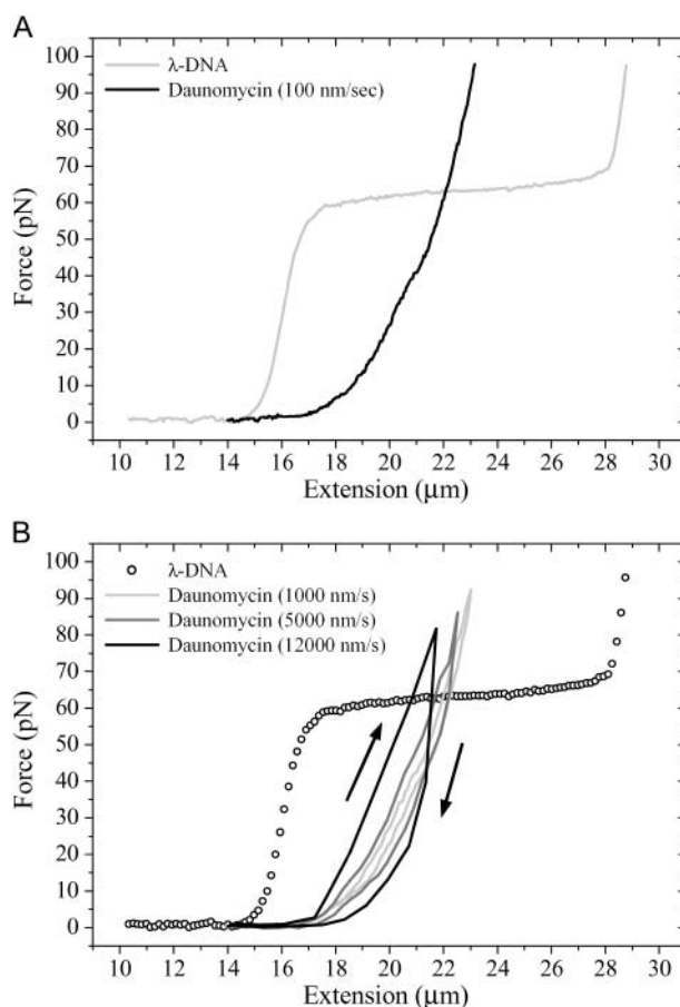
FIGURE 2 (A) Force-extension curves of a single \lambda -phage DNA molecule and in the presence of DNA intercalator daunomycin (1 \mu\text{M} ) obtained at a stretching velocity of 100 nm/s. (B) At higher velocities, daunomycin intercalated DNA reveals distinct hysteresis effects during extension-relaxation cycles.
