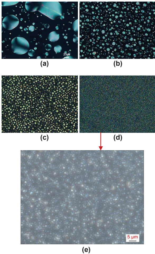
Figure 1. The microscopic images of PDLC droplets as a function of UV intensity; (a) UV intensity ( 0.2\mu\text{W cm}^{-2} ), (b) UV intensity ( 0.93\text{ mW cm}^{-2} ), (c) UV intensity ( 23.4\text{ mW cm}^{-2} ), (d) UV intensity ( 180\text{ mW cm}^{-2} ), and (e) enlarged microscopic image of the PDLC droplet (d).
