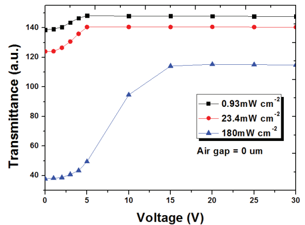
Figure 2. Transmittance-Voltage (TV) curve as a function of UV intensity such as 0.93\text{ mW cm}^{-2} , 23.4\text{ mW cm}^{-2} , and 180\text{ mW cm}^{-2} .
