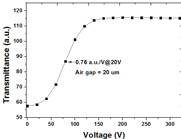
Figure 3. Transmittance-voltage (TV) curves of the EO modulator based on PDLC with a 20 \mu\text{m} air gap.
