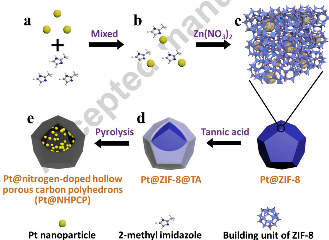
Fig. 1. Schematic illustration of the fabrication of Pt@NHPCP.
