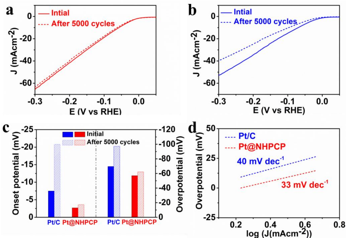
Fig. 4. Polarization curves of (a) commercial Pt/C and (b) Pt@NHPCP before and after 5000 potential cycles in 0.1 M HClO 4 solution with a sweep rate of 100 mV s -1 . (c) Onset potentials and overpotentials (at current density of 10.0 mA cm -2 ) of Pt@NHPCP and commercial Pt/C before and after 5000 potential cycles. (d) Tafel plots of Pt@NHPCP and commercial Pt/C after 5000 potential cycles.
