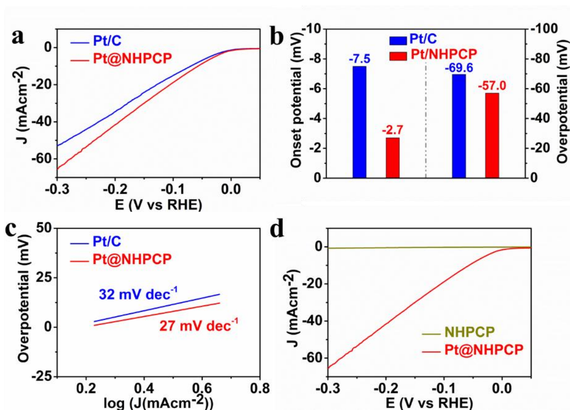
Fig. 3. (a) Polarization curves of Pt@NHPCP and commercial Pt/C for HER in 0.1 M HClO 4 with a potential scan rate of 5 mV s -1 . (b) Onset potentials and overpotentials (at current density of 10.0 mA cm -2 ) of Pt@NHPCP and commercial Pt/C. (c) Corresponding Tafel plots for the data presented in (a). (d) Polarization curves of Pt@NHPCP and pure NHPCP.
