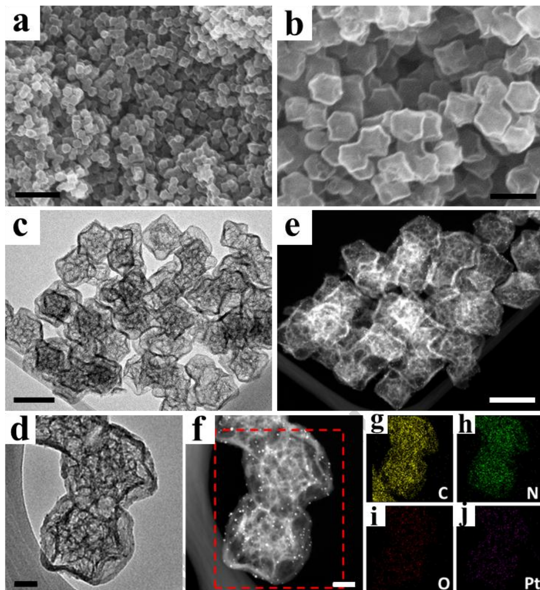
Fig. 2. (a) Low-resolution SEM, (b) high-resolution SEM, (c) low-resolution TEM, (d) high-resolution TEM, (e) low-resolution HAADF-STEM, and (f) high-resolution HAADF-STEM images of Pt@NHPCP. (g-j) Elemental mapping results of the zone indicated in (f): (g) C (yellow), (h) N (green), (i) O (red), and (j) Pt (purple). Scale bars are (a) 1 \mu m, (b) 300 nm, (c,e) 200 nm and (d,f) 50 nm.
