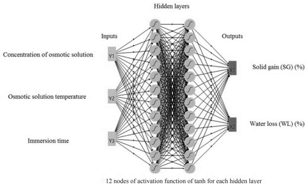
Fig. 1. Scheme of a neural network (concentration of osmotic solution ( y_1 ), osmotic solution temperature ( y_2 ), immersion time ( y_3 ), solid gain ( x_1 ), and dehydration ( x_2 )) with the arrangement of 3:12:12:2.
