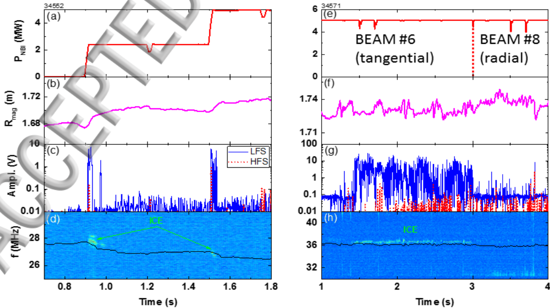
FIG. 3. Examples of core ICE at B_T = -1.79 T (discharge #34552, (a)-(d)) and B_T = -2.47 T (discharge #34571, (e)-(h)). D plasma and D beams. The plotted quantities are the NBI power P_{NBI} (a) and (e); the radial position of the magnetic axis R_{mag} (b) and (f); the amplitude of the RF signal on the low and the high field sides (LFS and HFS), on a logarithmic scale (c) and (g); and the frequency spectra of measured ICE intensity, on a logarithmic scale (d) and (h) (see (c) and (g) for relative scales, respectively). The black lines in (d) and (h) indicate the fundamental hydrogen cyclotron frequency calculated at the magnetic axis.
