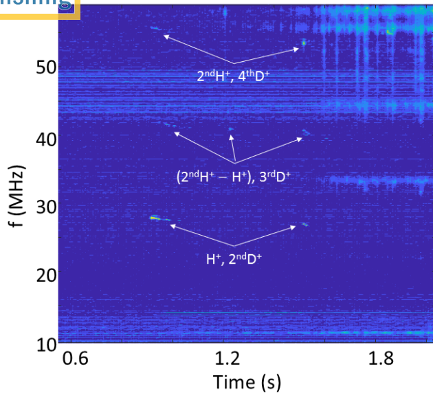
FIG. 4. ICE frequency spectrum for the discharge shown in Fig. 3 (a)-(d).
