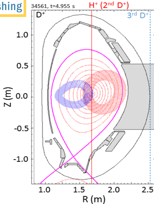
FIG. 6. Frequency matched radial positions of the fundamental deuterium (dotted black line), the fundamental hydrogen (solid red line), and the third harmonic deuterium (dashed blue line) cyclotron frequencies for discharge 34561 in FIG. 5. The two shown orbits correspond to barely confined fusion proton orbits. Both orbits originate at the magnetic axis.
