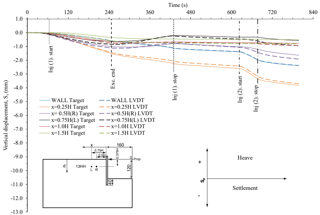
Figure 6. 18 Retained surface vertical displacements measured by LVDTs and image processing targets (15 mm below the surface) in test 13HH above the wall and at distances x=0.25H , 0.5H , 0.75H , 1.0H and 1.5H behind the wall.
