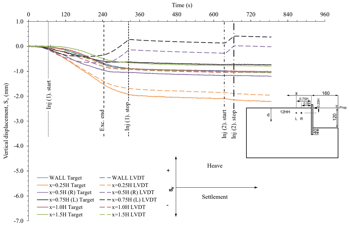
Figure 6.13 Retained surface vertical displacements measured by LVDTs and image processing targets (15 mm below the surface) in test 12HH above the wall and at distances x=0.25H , 0.5H , 0.75H , 1.0H and 1.5H behind the wall.
