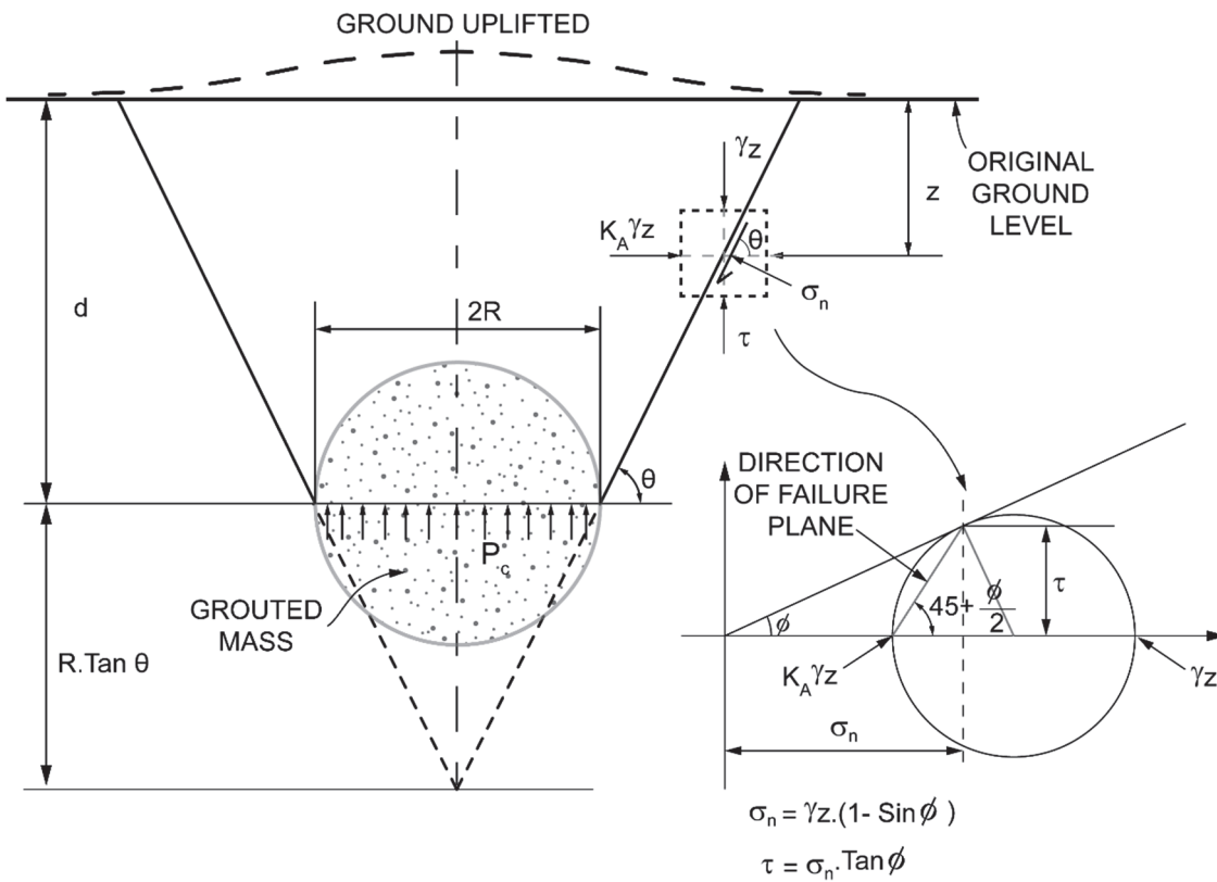
Figure 3. 8 Conical shearing failure above spherical grout bulb (after Wong, 1974).
