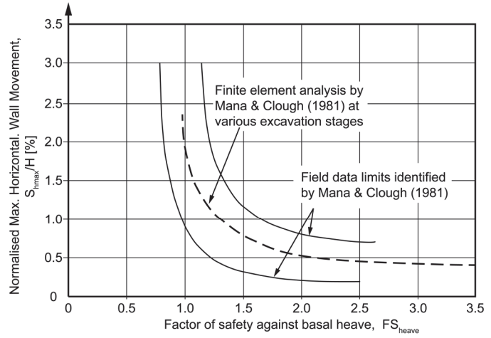
(b) Relationship between factor of safety against basal heave and normalised maximum horizontal wall movement (after Mana & Clough, 1981)
