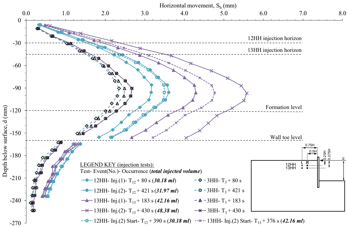
Figure 6. 56 Horizontal wall movements at the end of the injection events in tests 12-13HH (and start of the 2 nd injection events) compared to equivalent stages in baseline test 3HH.
