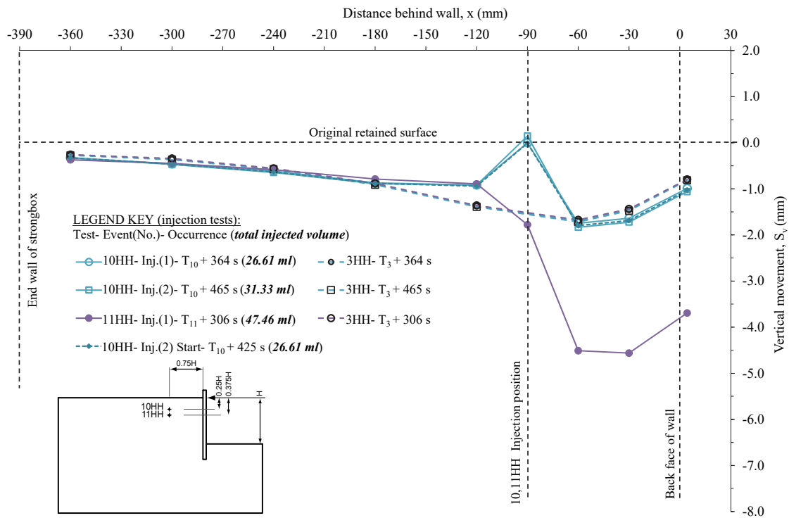
Figure 6. 47 Vertical LVDT retained surface displacements at the end of the injection events in tests 10-11HH (and start of the 2 nd injection event in test 10HH) compared to equivalent stages T 3 in baseline test 3HH.
