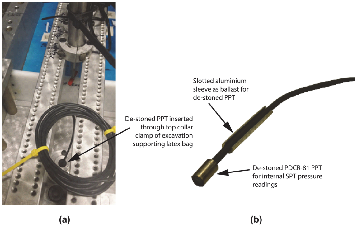
Figure 5.36 Photographs showing: (a) insertion of the de-stoned Druck PDCR-81 PPT and (b) the slotted ballast sleeve attached behind the de-stoned PPT to ensure its positioning at the bottom of the SPT filled excavation support latex bag.
