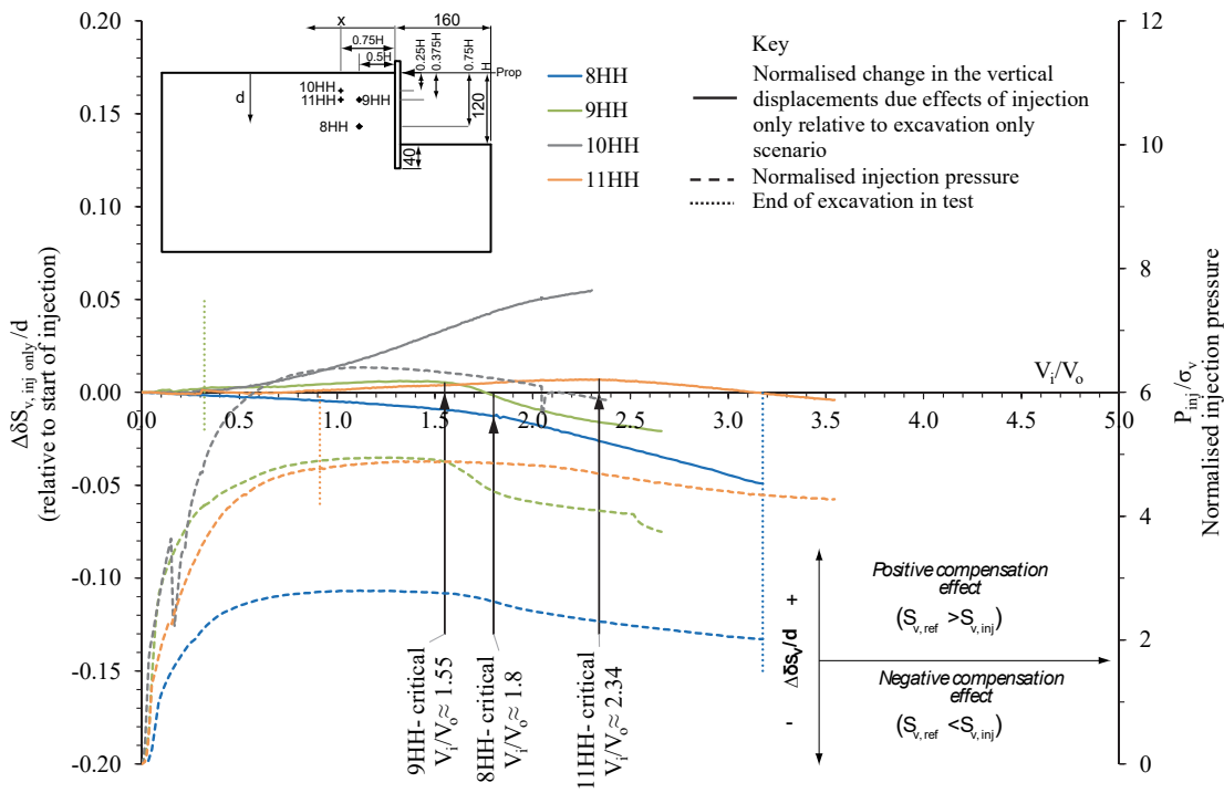
Figure 7.3 Normalised changes in vertical displacements and injection pressures with injected volume above the injection location relative to the reference test from the start of injection in tests 8HH, 9HH, 10HH and 11HH.
