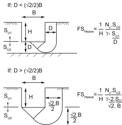
(a) Calculation of factor of safety against basal heave (after Terzaghi, 1943; Bjerrum & Eide, 1956)
