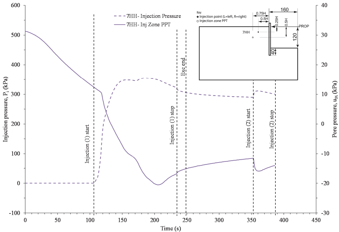
Figure 6. 60 Injection pressure and locally installed injection zone PPT response during test 7HH.
