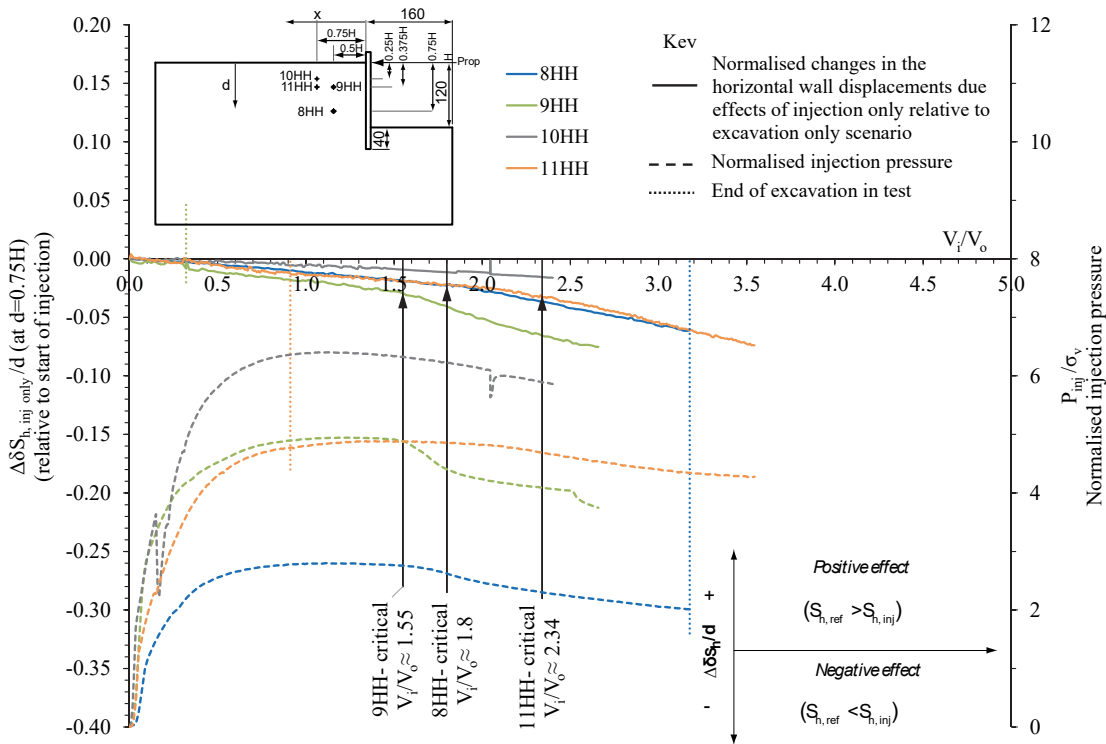
Figure 7.4 Normalised changes in horizontal wall displacements at depth d=0.75H , below the retained surface and injection pressures with injected volume, relative to the reference test from the start of injection in tests 8HH, 9HH, 10HH and 11HH.
