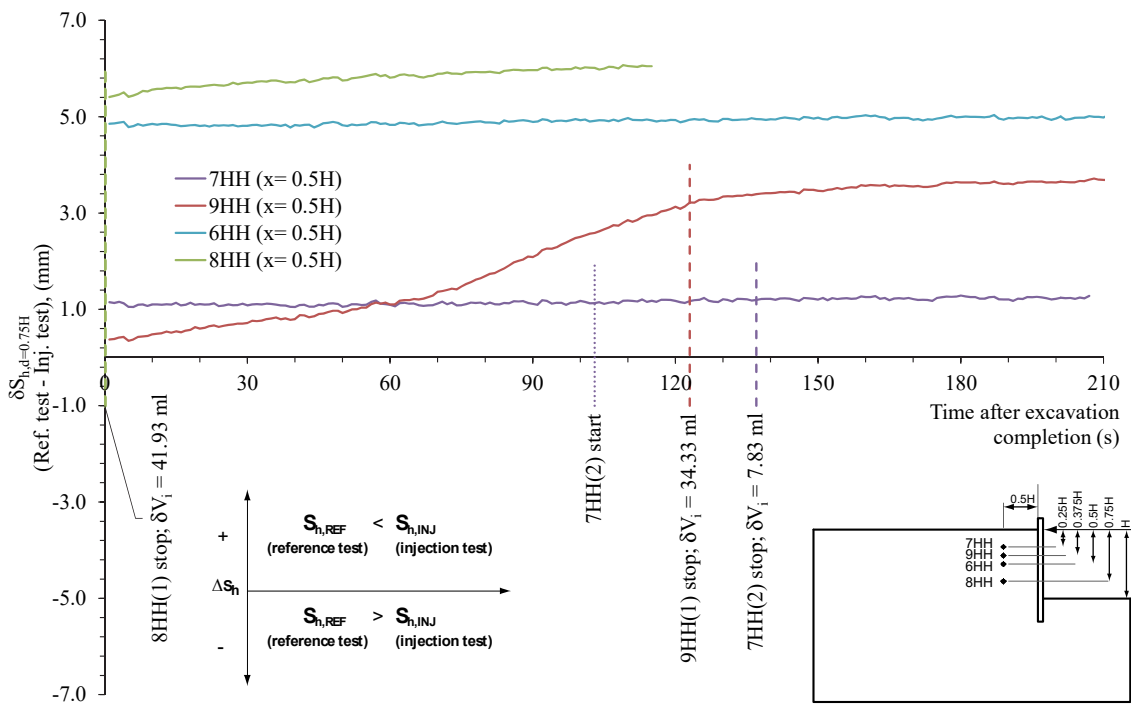
Figure 7. 16 Development of horizontal wall displacements at depth d=0.75H , below the retained surface, in grouting tests 6-9HH relative to test 3HH after the simulated excavation.
