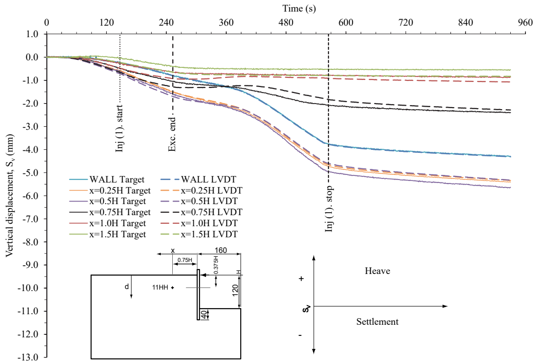
Figure 6. 17 Retained surface vertical displacements measured by LVDTs and image processing targets (15 mm below the surface) in test 11HH above the wall and at distances x=0.25H , 0.5H , 0.75H , 1.0H and 1.5H behind the wall.
