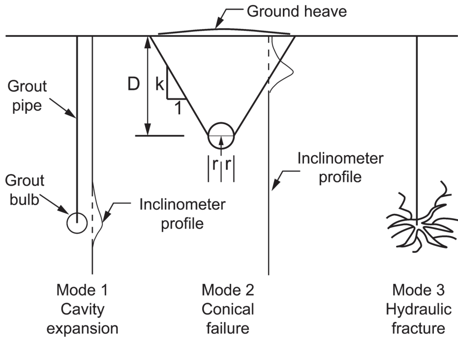
Figure 3. 7 Modes of soil mass deformation by compaction grouting (after Wong et al. , 1996).
