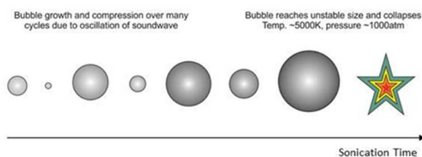
Fig. 3 Growth and collapse of bubbles, arising from acoustic cavitation. Once the bubble reaches an unstable size it collapses, giving enormous local temperatures and pressures.
