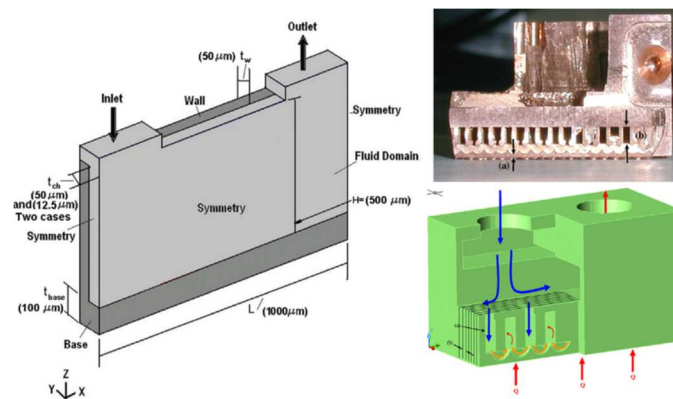
Fig. 15 Design concept and cross-sectional view of microchannel heat exchanger. 192
