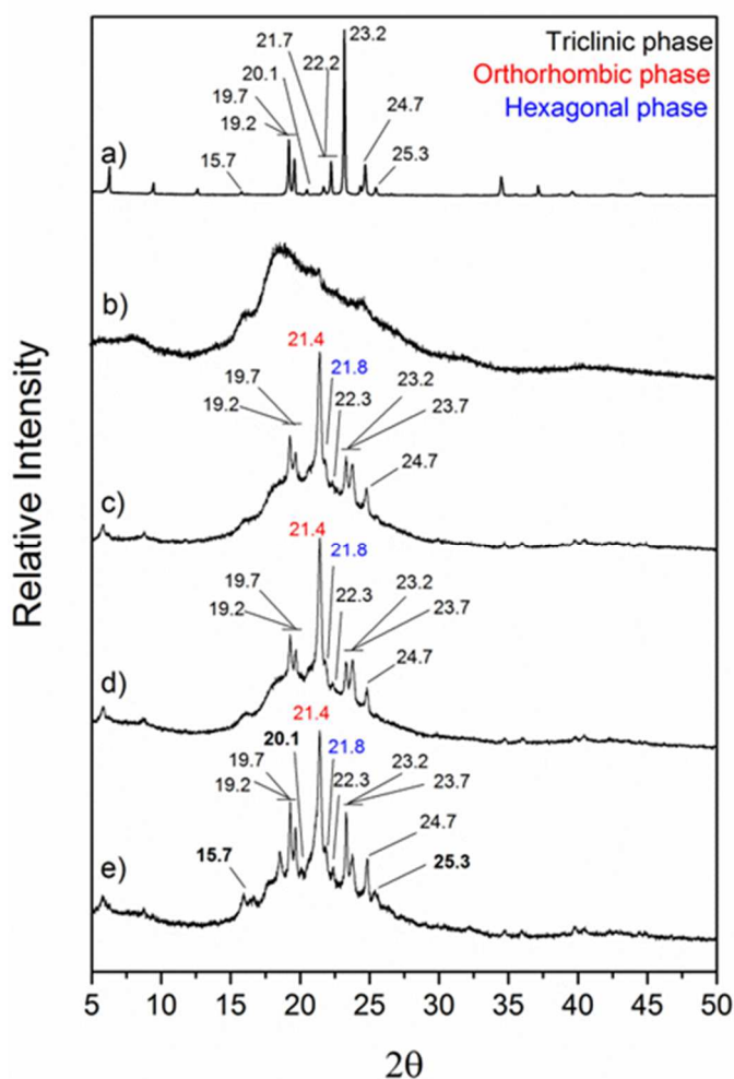
Fig. 7 X-ray diffractograms of a) bulk n-docosane, b) polyurethane shell (hollow microcapsules), n-docosane loaded into c) 10 \mu\text{m} microcapsules, d) 4 \mu\text{m} microcapsules and e) 2 \mu\text{m} microcapsules. 130
