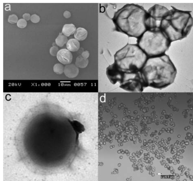
Fig. 11 (a) - SEM, (b, c) - TEM, and (d) - optical microscopic images of the eicosane/EC/MC capsules prepared with a 9 wt.% polymer content. 160
