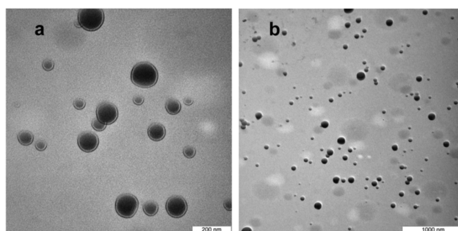
Fig. 8 TEM images of the n-octadecane/polystyrene/(PMMA) capsules at (a) 100k magnification and (b) 30k magnification. 143
