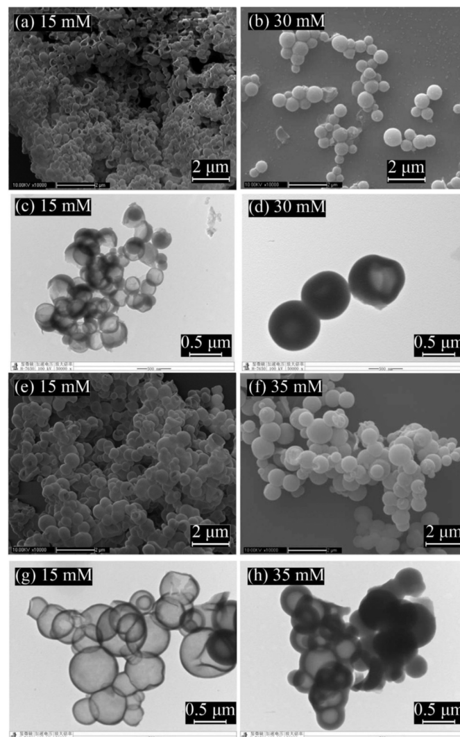
Fig. 9 (a, b, e, f) SEM and (c, d, g, h) TEM images of the silica nanocapsules loaded with n-octadecane prepared at different CTAB concentrations. 152
