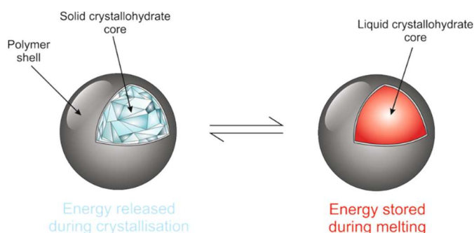
Fig. 12 Cartoon showing ideal capsule behaviour for the salt hydrate core. 173
