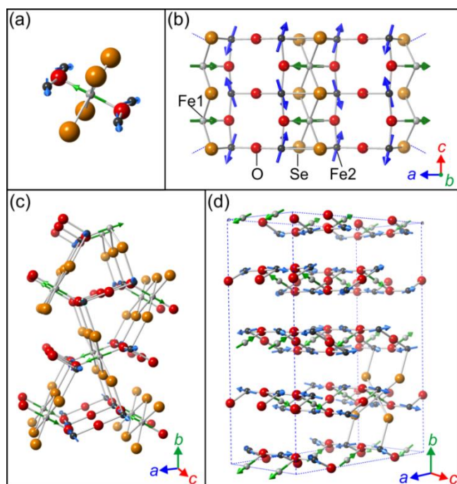
Figure 11. Magnetic structure of \text{Sr}_2\text{Fe}_3\text{Se}_2\text{O}_3 observed between 1.5 and 50 K ( T_{N2} ). (a) the local environment of the Fe1 moment relative to the nearest neighbour Fe2 sites. (b) Arrangement of Fe1 and Fe2 moments in the spin hybrid ladders (compare with Figure 7(b)). (c) Arrangement of moments between ladders. (d) magnetic unit cell below T_{N2} , which is a 2a \times 2b \times 2c expansion relative to the nuclear cell (see Table S6). Sr and most Se sites not shown in (d) for clarity.
