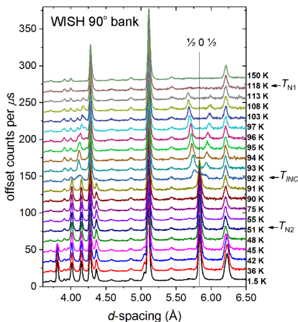
Figure 5. Evolution with temperature of the neutron powder diffraction patterns of Sr 2 Fe 3 Se 2 O 3 sample A measured as a function of temperature. Data from the detector bank with a mean 2θ of 90° are shown.
