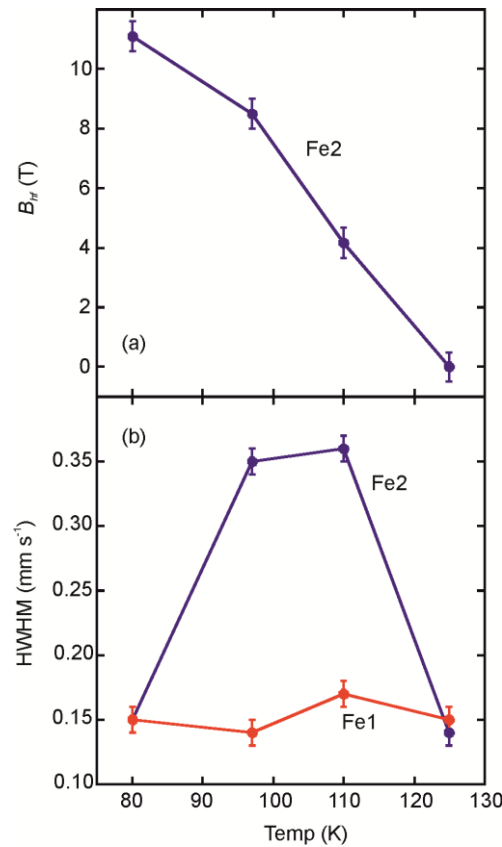
Figure 14. (a) The evolution of the mean hyperfine field, B_{hf} , for the Fe2 sites on cooling through T_{N1} and T_{INC} . (b) The evolution of the linewidths (expressed as half-width at half-maximum (HWHM)) for the Fe1 and Fe2 signals on cooling through T_{N1} and T_{INC} . The broader widths in the region of the incommensurate spin density wave order of the Fe2 moments are ascribed to the range of hyperfine fields experienced by these sites. See Table 2.
