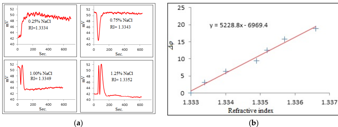
Figure 3. Evaluation of refractive index sensitivity: (a) response signals to refractive index changing, (b) dependence of phase shift (in rad) against refractive index.
