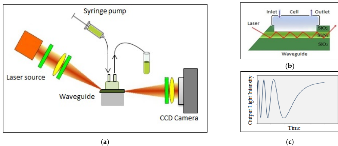
Figure 1. Designs of (a) planar waveguide and (b) polarization interferometer (PI) experimental setup; (c) expected output signal waveform.
