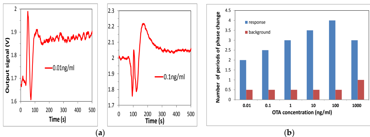
Figure 4. (a) Typical sensor responses to binding of 0.01 ng/mL and 0.1 ng/mL of ochratoxin A (OTA) to specific antibodies; (b) dependence of PI sensor response on concentration of OTA.
