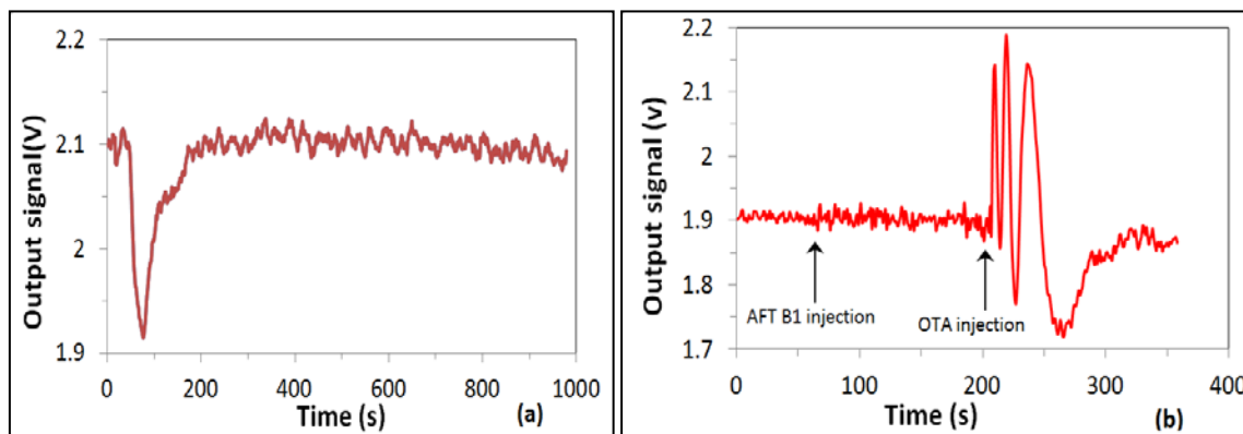
Figure 5. Control tests: (a) typical PI sensor response to washing out nonspecifically bound OTA (1 ng/mL), (b) typical response to injection of nontargeted analyte, aflatoxin B1 (1 ng/mL); response to injection of 1 ng/mL of OTA is given for comparison. Negative control tests were also carried out by injecting a different toxin (aflatoxin B1), which is not supposed to be bound to anti-OTA antibodies. As shown in (b), the response to aflatoxin B1 was comparable to the noise level, indicating high specificity of OTA detection.
