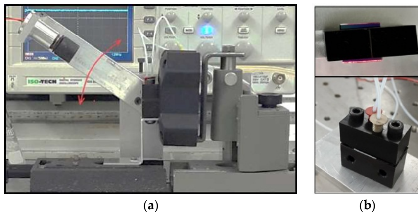
Figure 2. Photographs of (a) PI experimental setup and (b) reaction cell with inserted waveguide.
