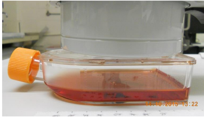
Figure 6.6: Experimental set up of the system uniformity and sensitivity tests. The camera head was positioned above the flask containing the flood source (mixture of ^{99m}\text{Tc} solution and red coloured dye).
