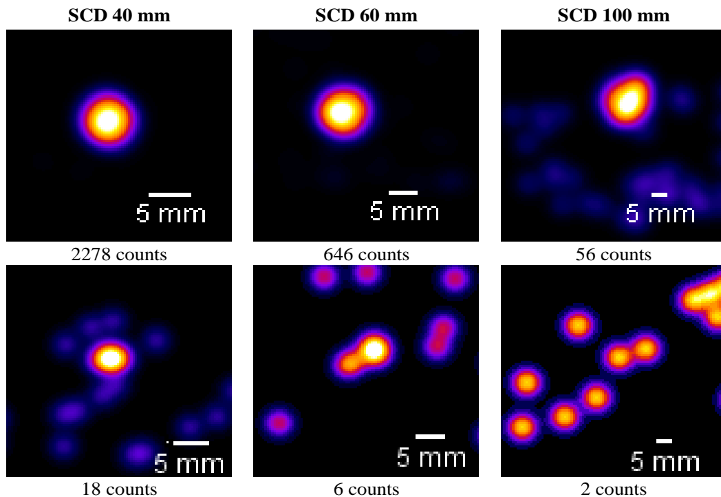
Figure 5.18: Relationship between CNR and SCDs for images acquired using 1 mm (top row) and 0.5 mm (bottom row) pinhole collimators. The number of counts within the ROI of the seed were indicated underneath of each images ( n=3 ).
