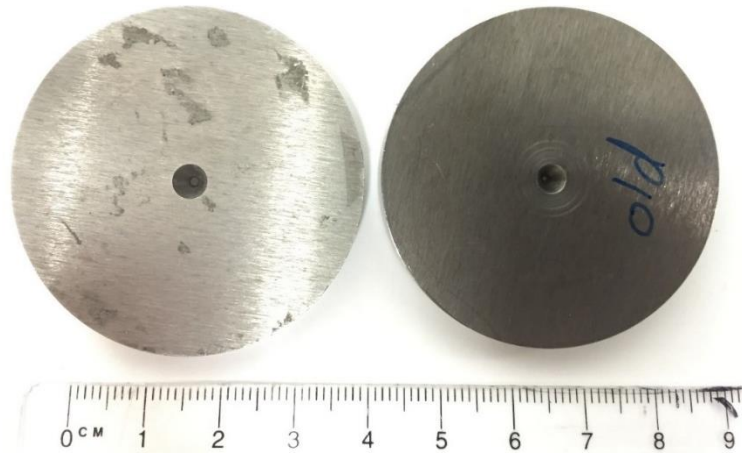
Figure 2.11: Bespoke pinhole collimator for HGC with pinhole diameters of 1 mm (left) or 0.5 mm (right).
