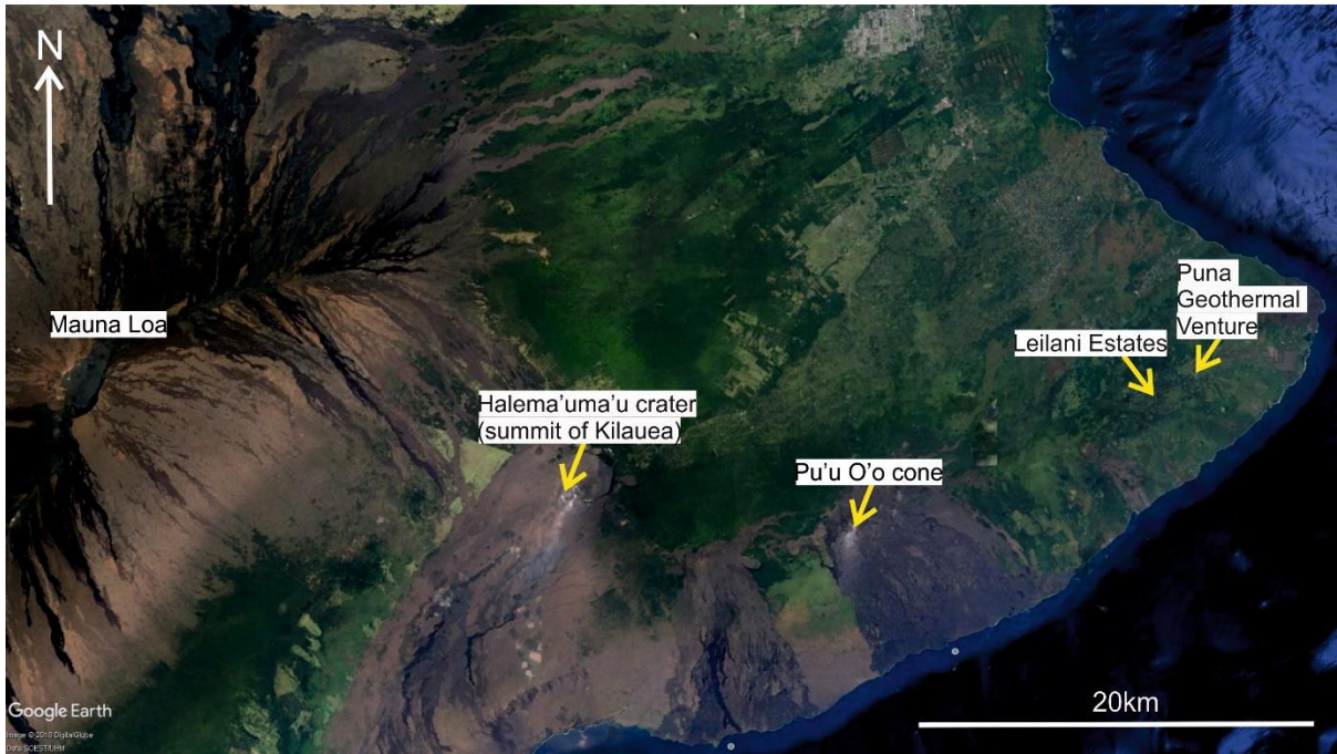
Fig.1. The East Rift Zone of Kīlauea volcano runs from the summit area (Halema'uma'u crater) to Pu'u 'Ō'ō cone to the site of current activity in the lower East Rift Zone, centred in the Leilani Estates area and have encroached on a geothermal energy plant known as the Puna Geothermal Venture (PGV) (image courtesy of Google Earth)
