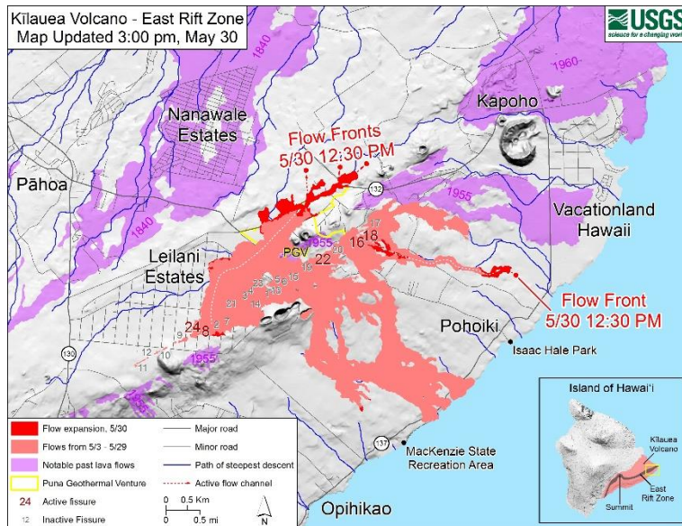
Fig. 3 Map of lava flows erupted from fissures on the Lower East Rift Zone (LERZ) of Kilauea as of May 30 th 2018. Note the geothermal plant (PGV), which is at the time of writing partly covered by lavas from fissures 7 and 8. The area of property damage in the Leilani Estates, where at least 25 homes have been destroyed to date, and the ocean entry points of lavas are also shown. The inset shows the location of Kilauea on the south-east flank of Mauna Loa volcano, the East Rift Zone and the summit crater of Halema'u ma'u. (map courtesy of USGS/Hawai'ian Volcano Observatory)
