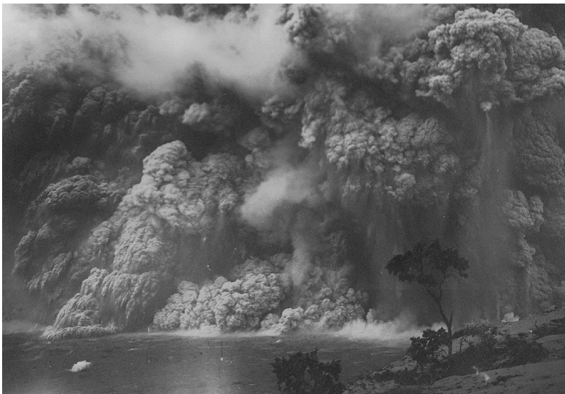
Fig. 7. Pyroclastic density currents flowing away from the base of a plume of ash during the 1924 phreatomagmatic eruptions at the summit of Kīlauea. A similar eruption but large volume eruption around 1790 killed at least 80 Hawai'ians (image courtesy of the Bishop Museum, Hawai'i)
