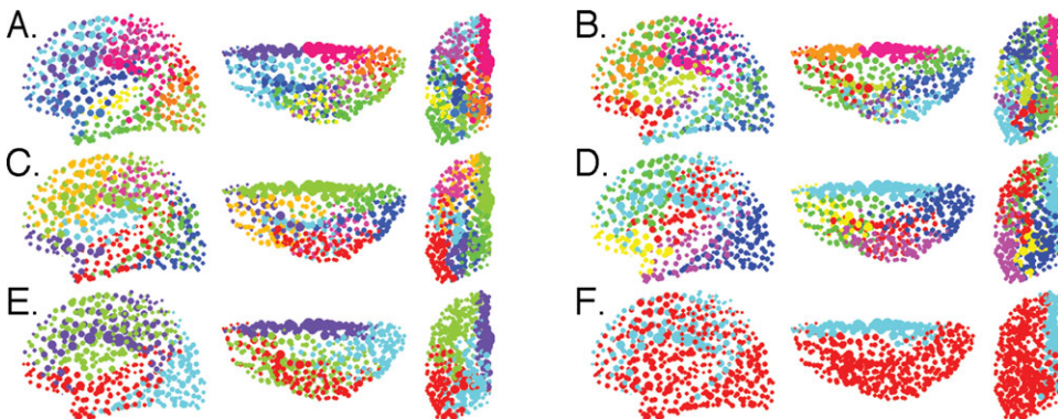
Fig. 4. Consensus partitions obtained at different Markov times; (A) t \approx 10^{-0.23} with 12 communities; (B) t \approx 10^{0.08} with 10 communities; (C) t \approx 10^{0.273} with eight communities; (D) t \approx 10^{0.53} with six communities; (E) t \approx 10^{0.76} with four communities; (F) t \approx 10^{2.89} with two communities. Vertex size is proportional to strength. (Color online)
